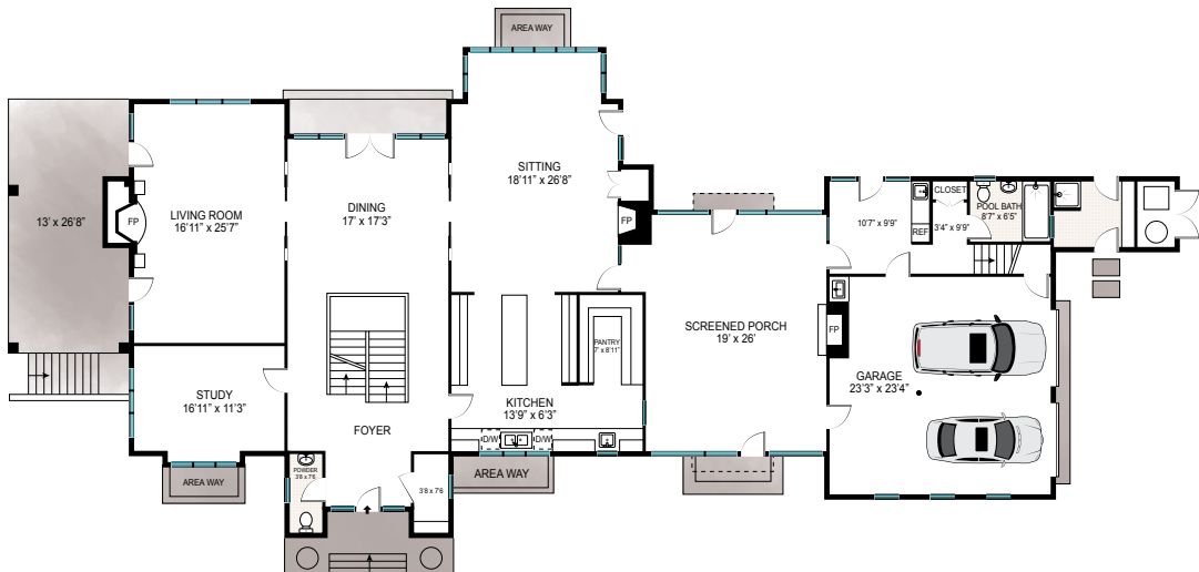
FIRST FLOOR
