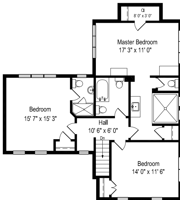
SECOND FLOOR
