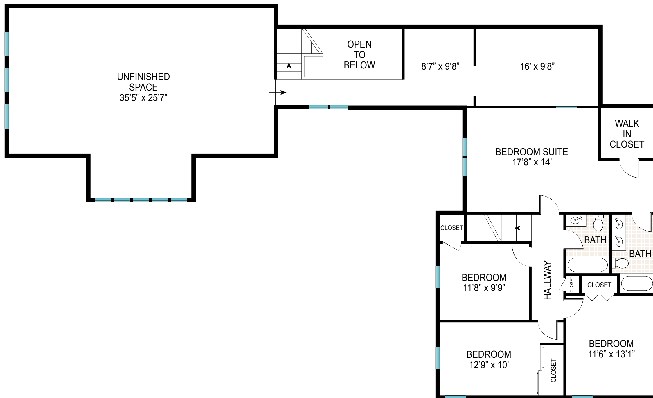
SECOND FLOOR
