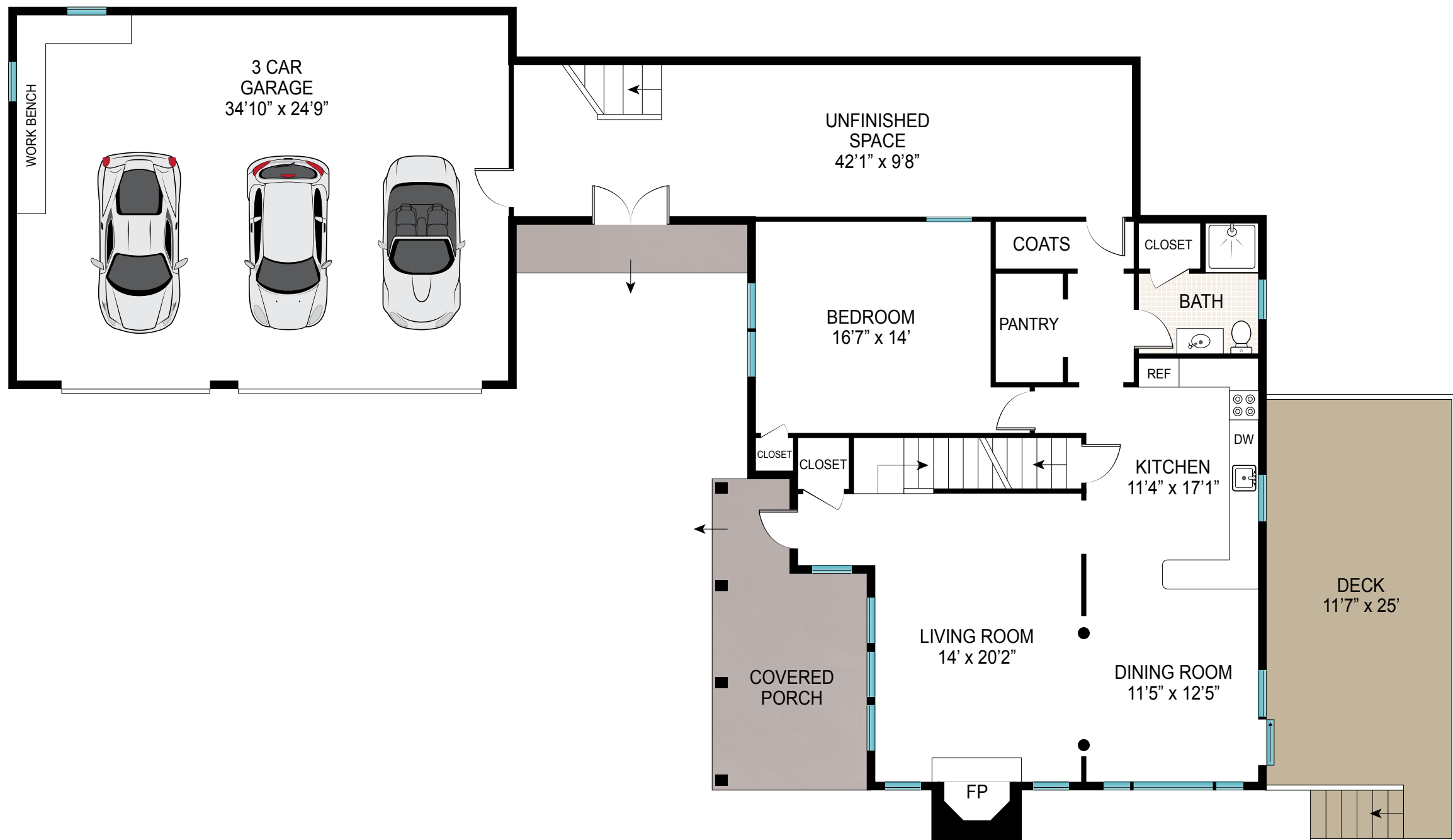
FIRST FLOOR
