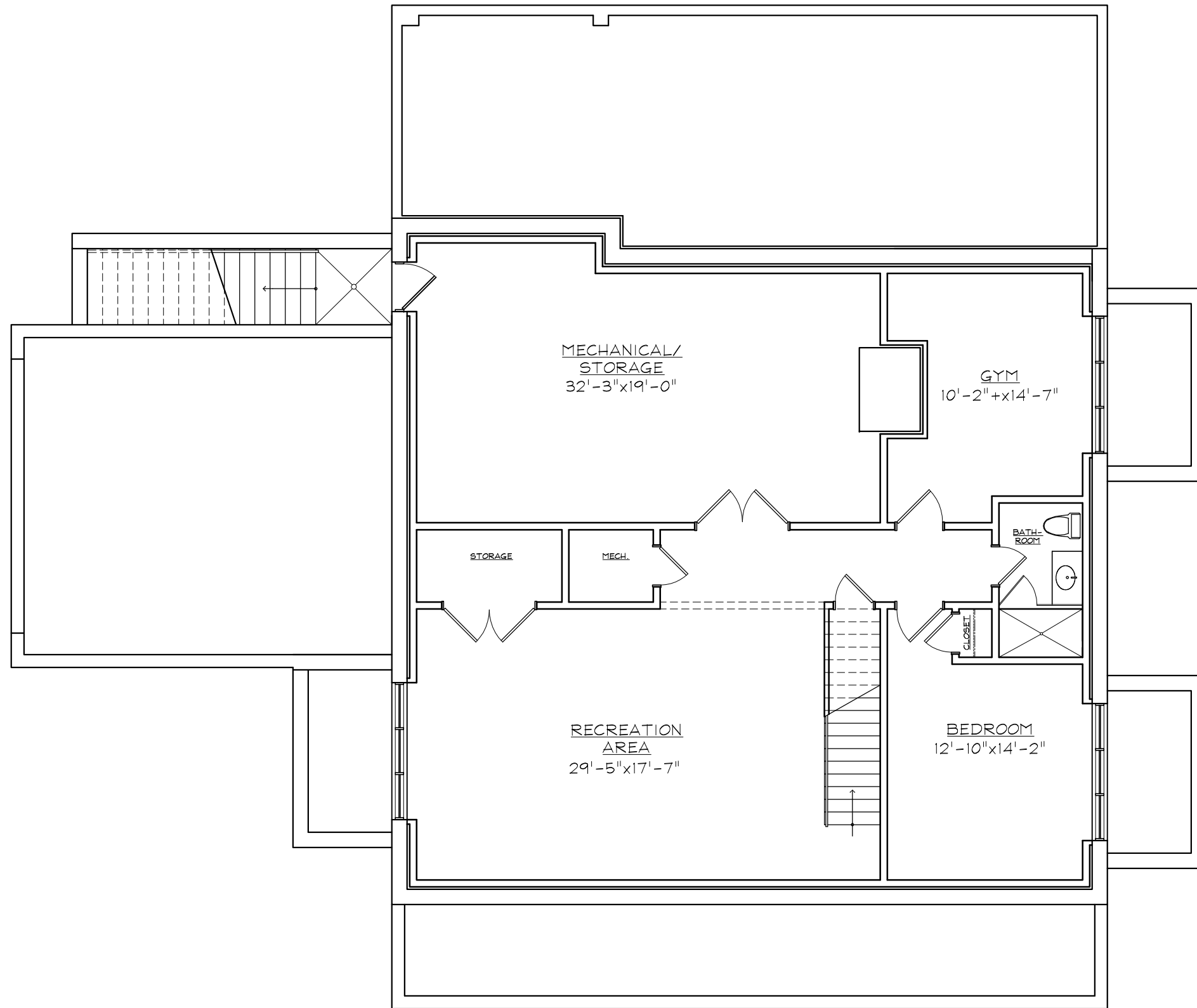
BASEMENT PLAN RUGGS PATH (LOT #2)
