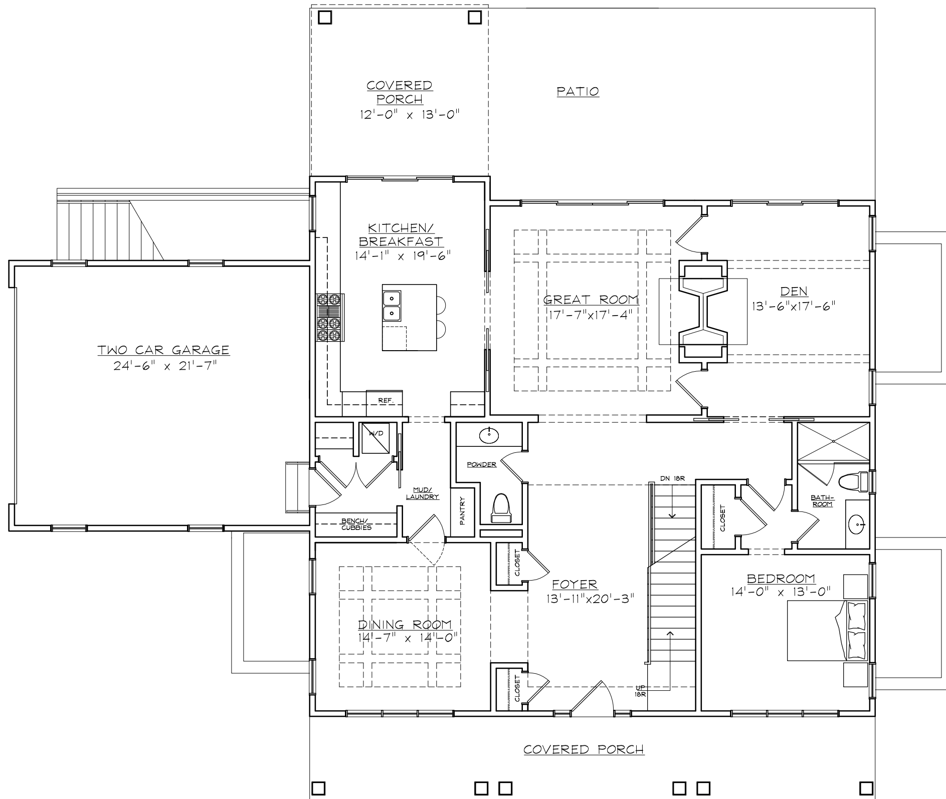
FIRST FLOOR PLAN RUGGS PATH (LOT #2)
