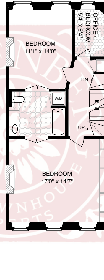
SECOND FLOOR 9'9" HEIGHT CEILING
