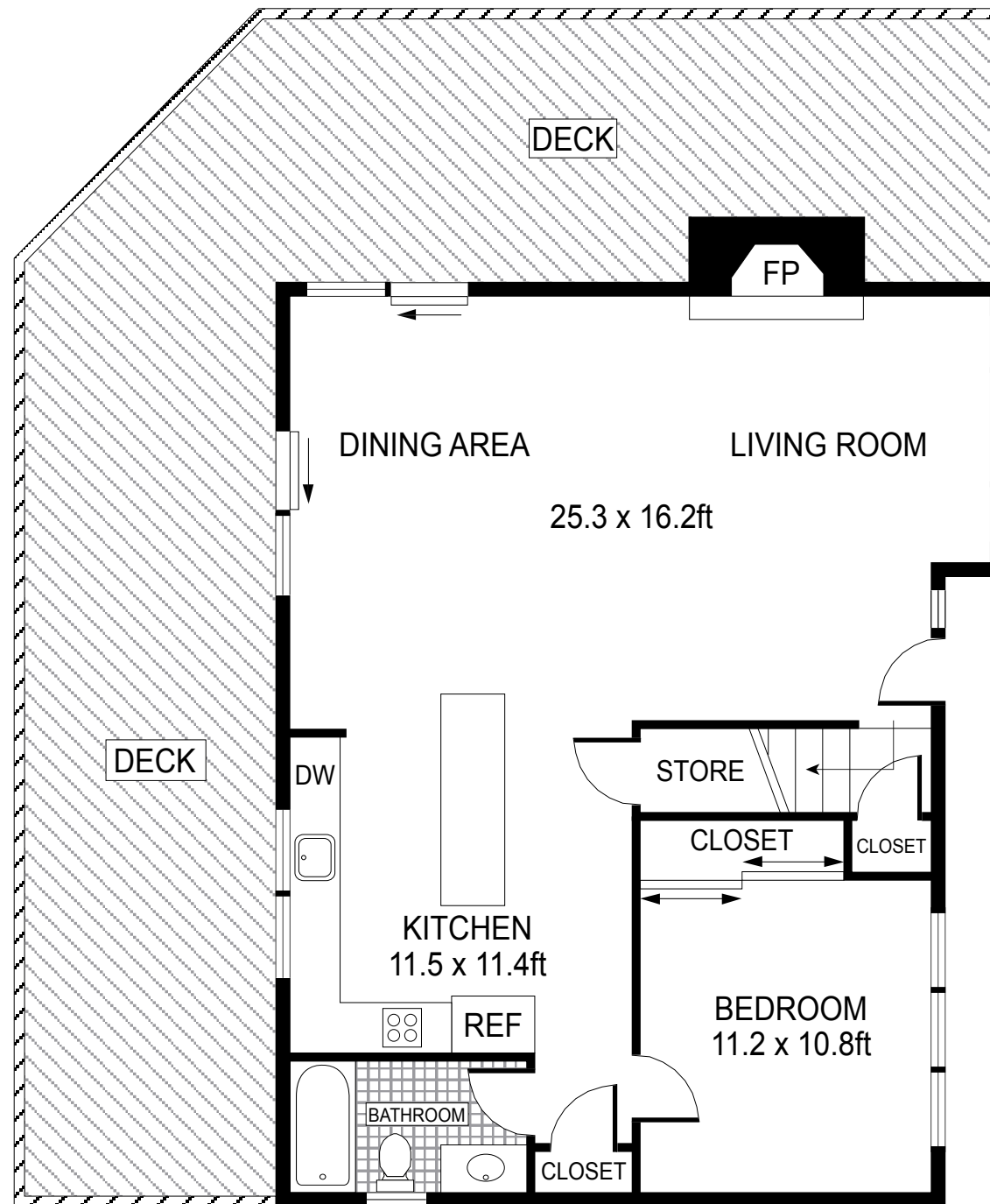
FIRST FLOOR
