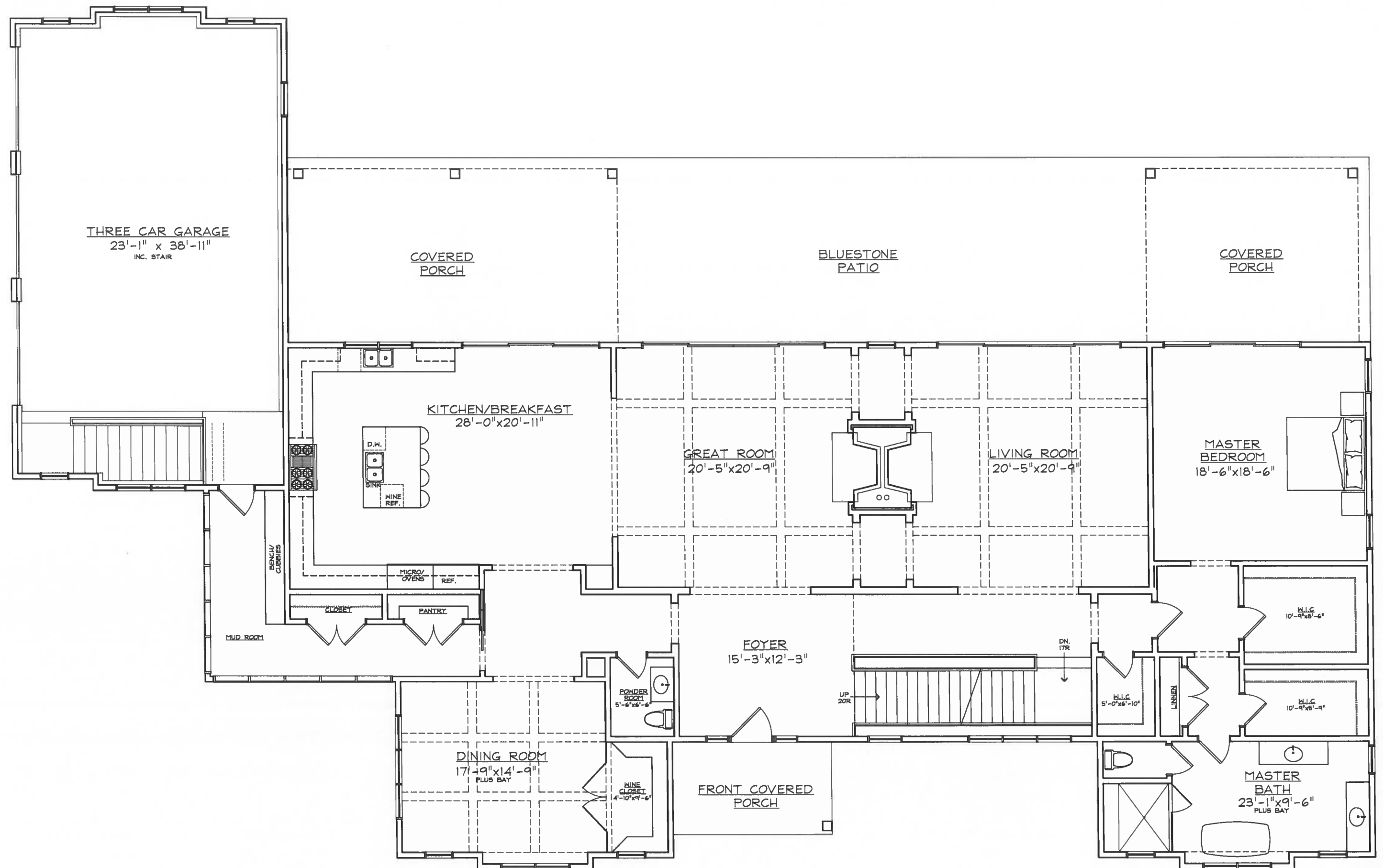
FIRST FLOOR PLAN (5-20-15) POLO COURT LOT 2
