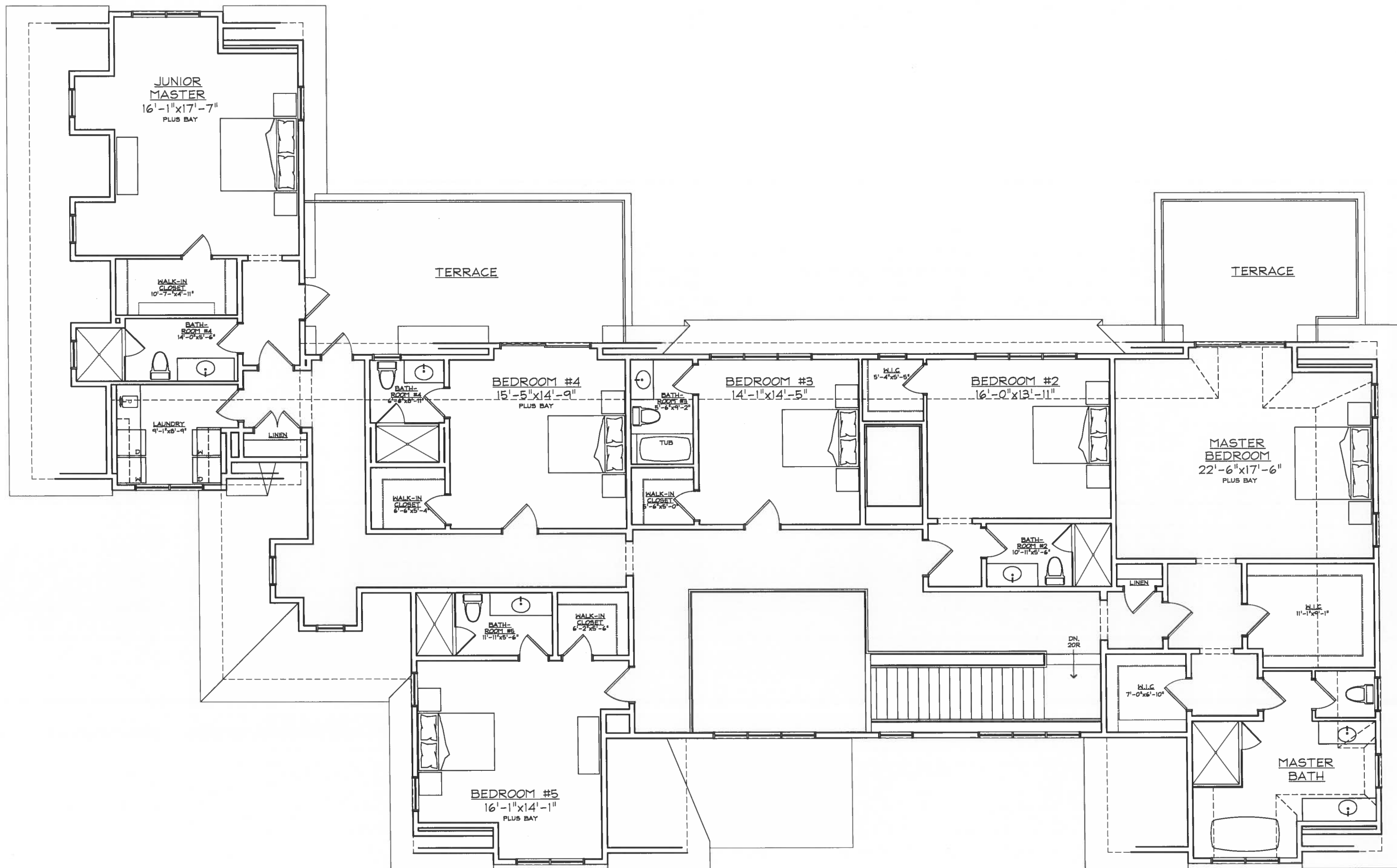
SECOND FLOOR PLAN (5-20-15) POLO COURT LOT 2
