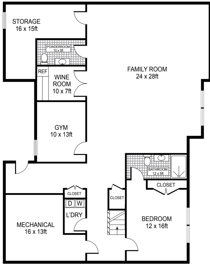
LOWER FLOOR
