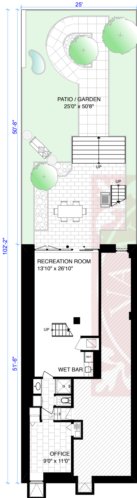
TRIPLEX / GARDEN FLOOR 7'4" / 7'10" HEIGHTS CEILINGS
