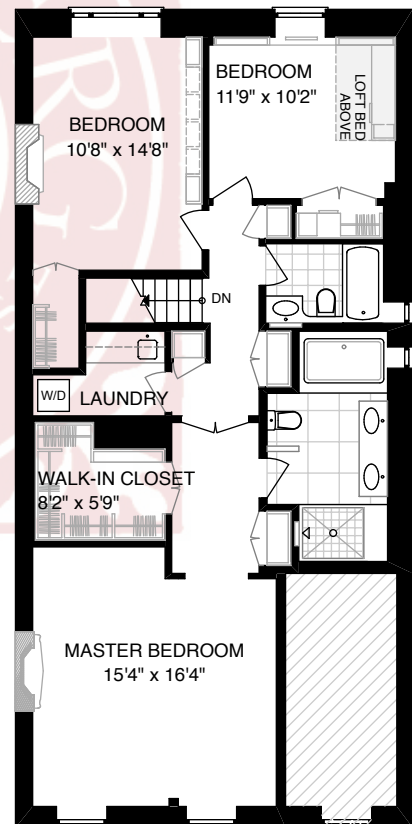
TRIPLEX / SECOND FLOOR 11'0" HEIGHTS CEILINGS
