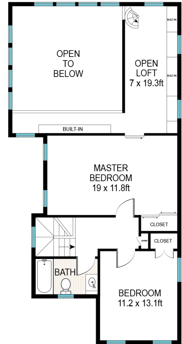
SECOND FLOOR
