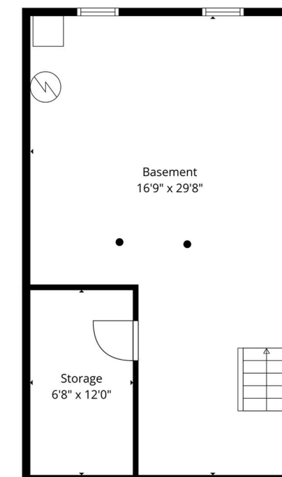
BASEMENT
