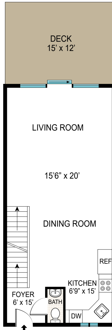
FIRST LEVEL CEILING HEIGHT: 7'10"
