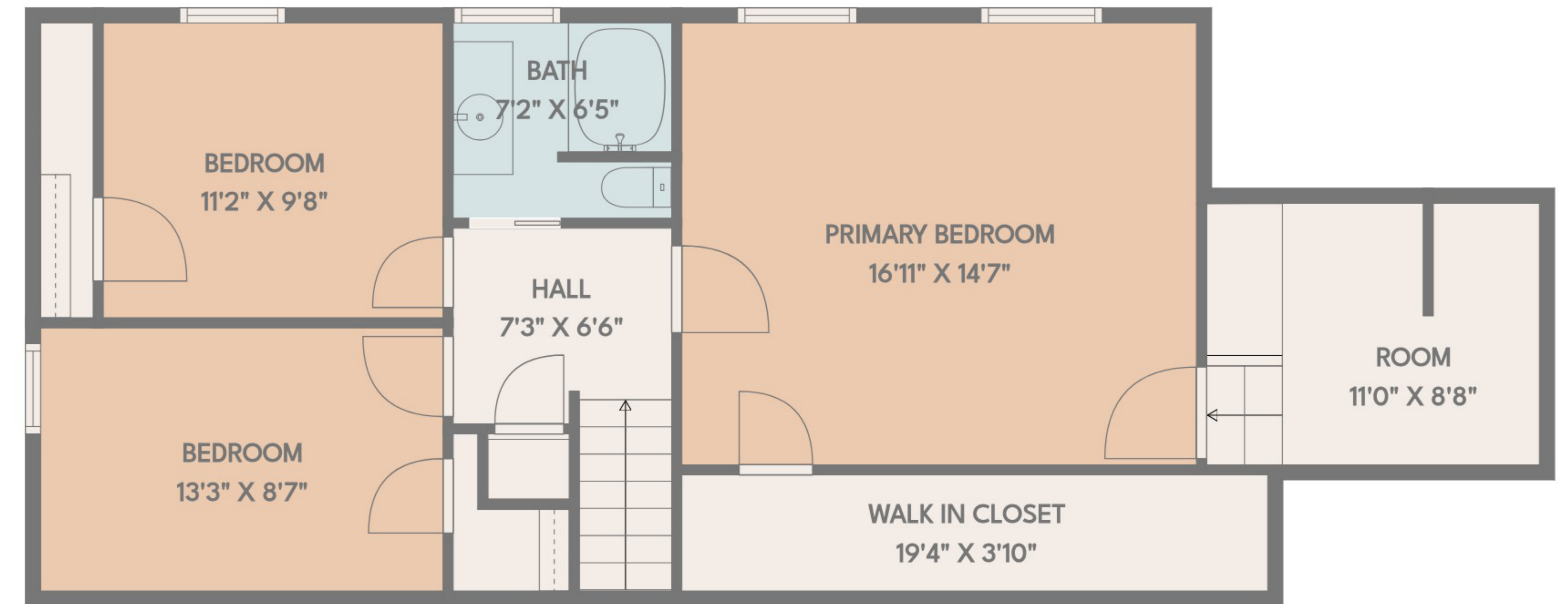
SECOND FLOOR
