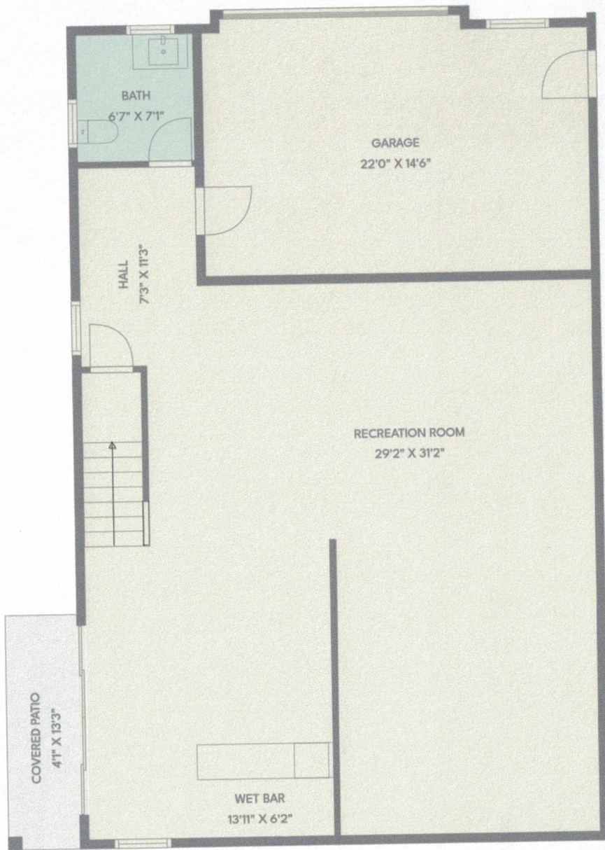
1ST FLOOR
