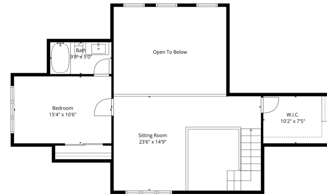
SECOND FLOOR
