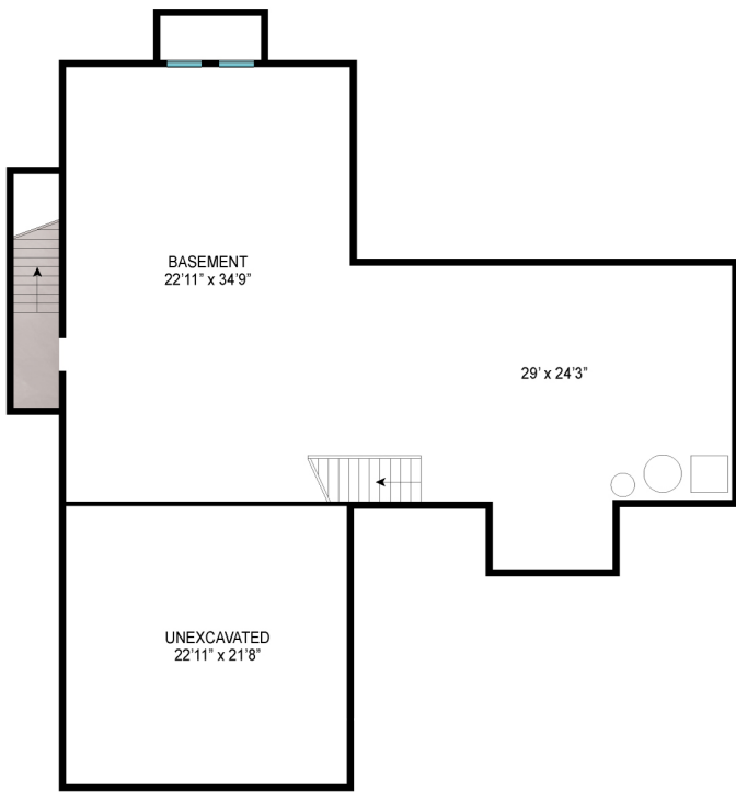
BASEMENT
