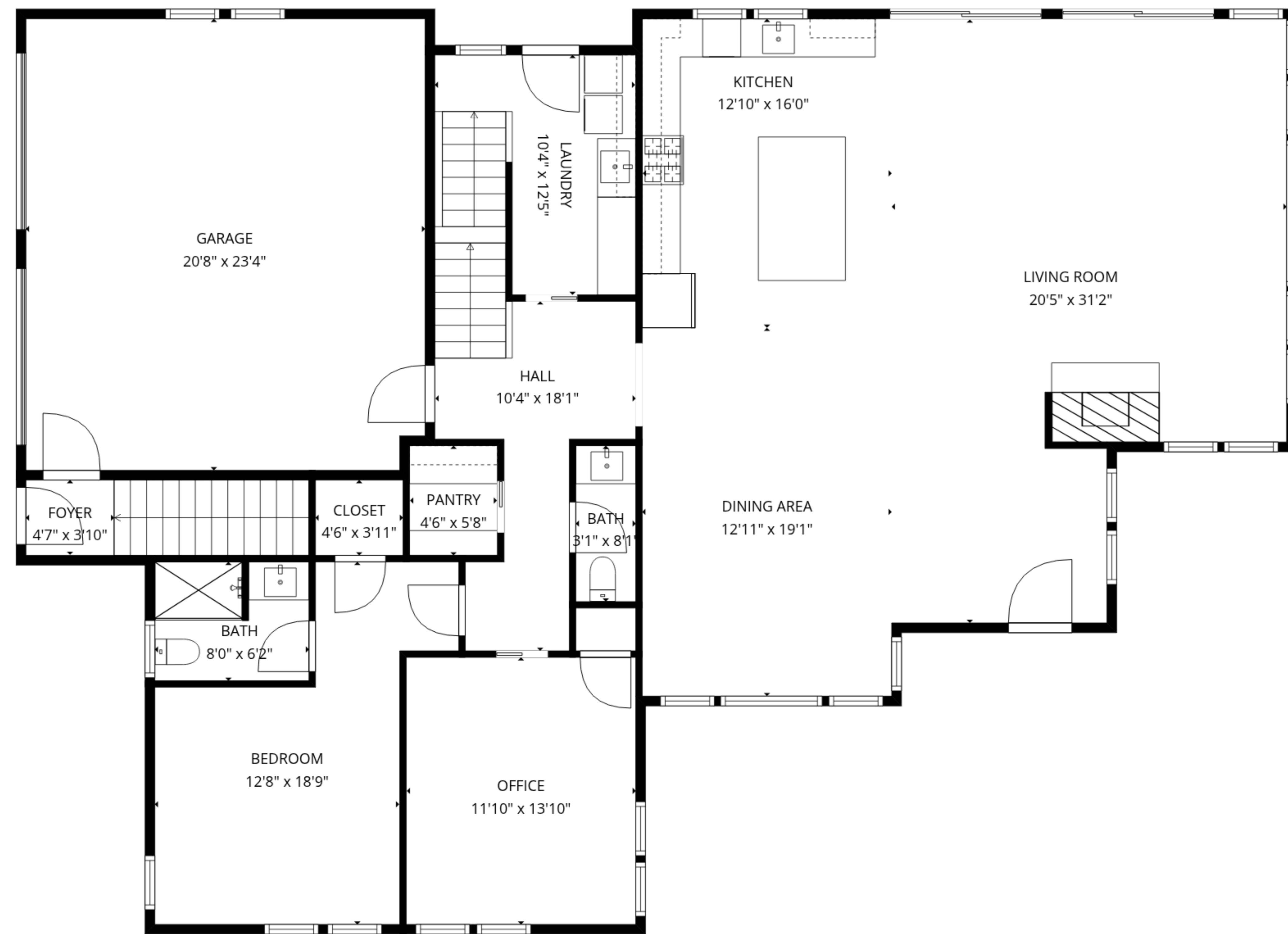
FLOOR 2
