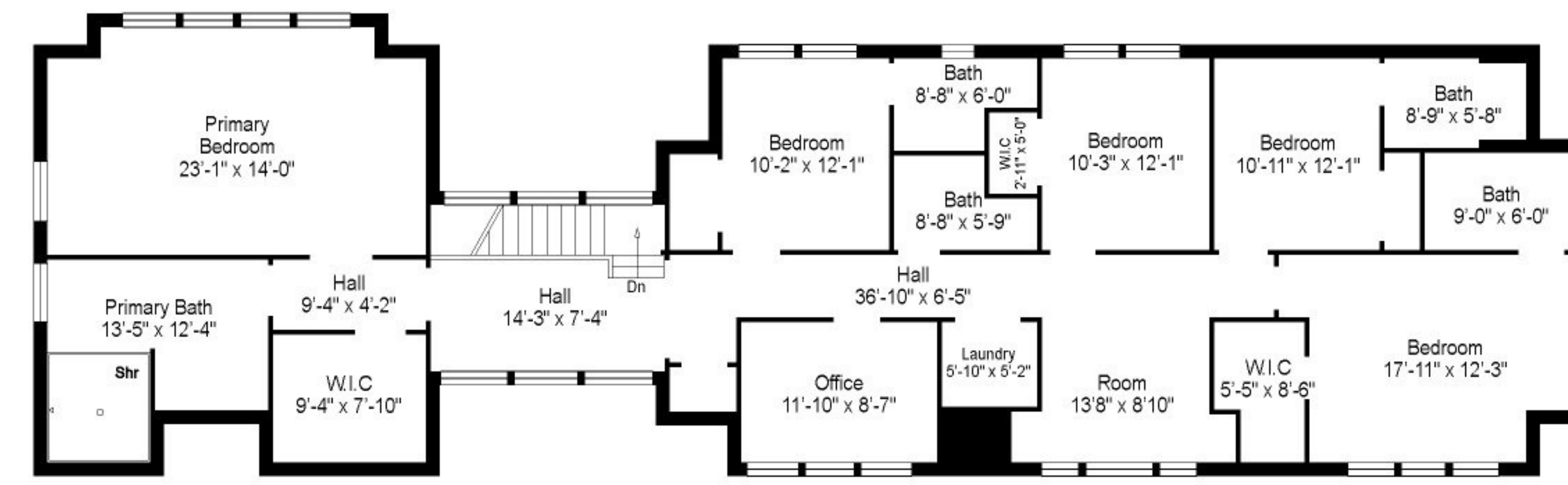
SECOND FLOOR
