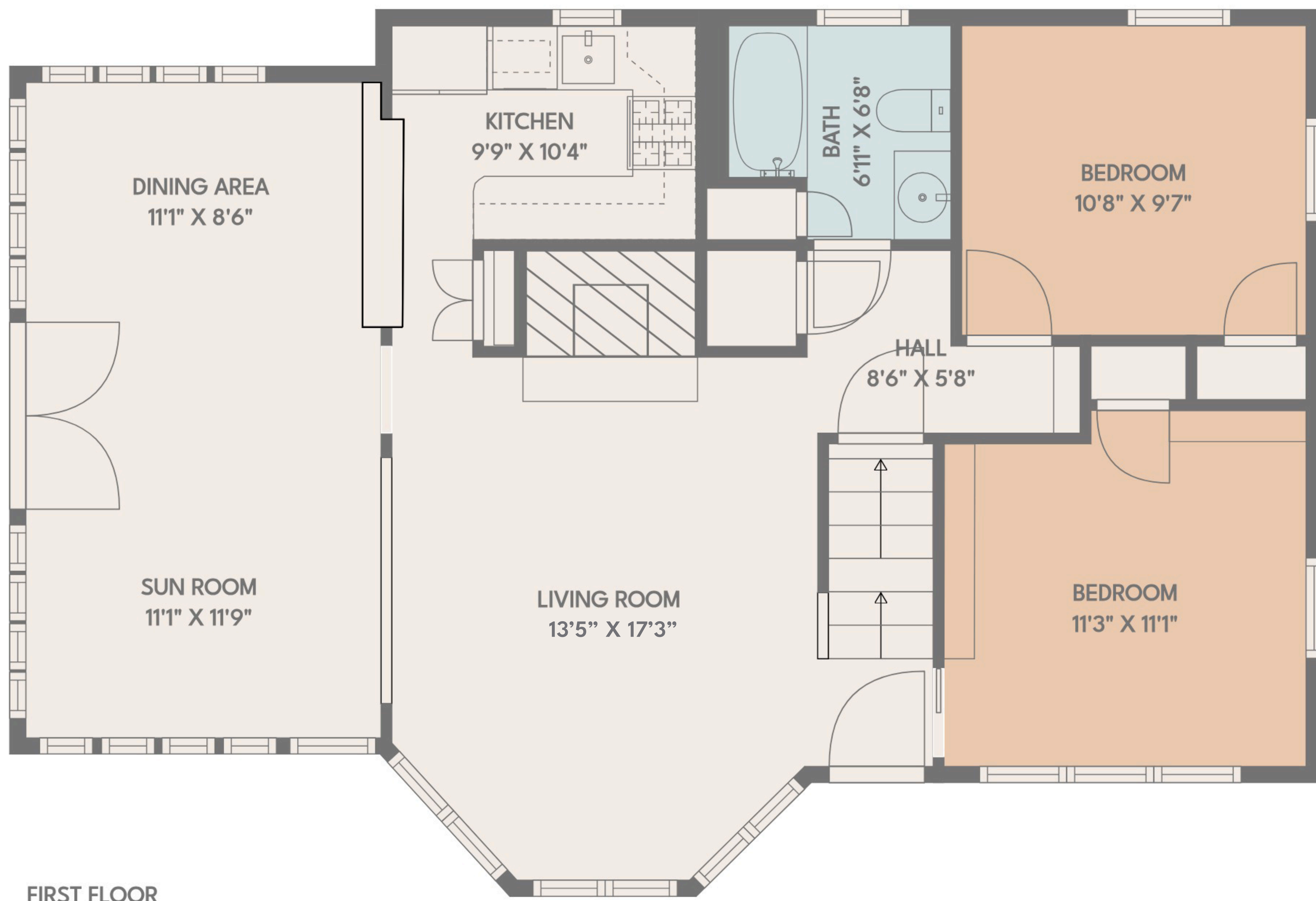
FIRST FLOOR
