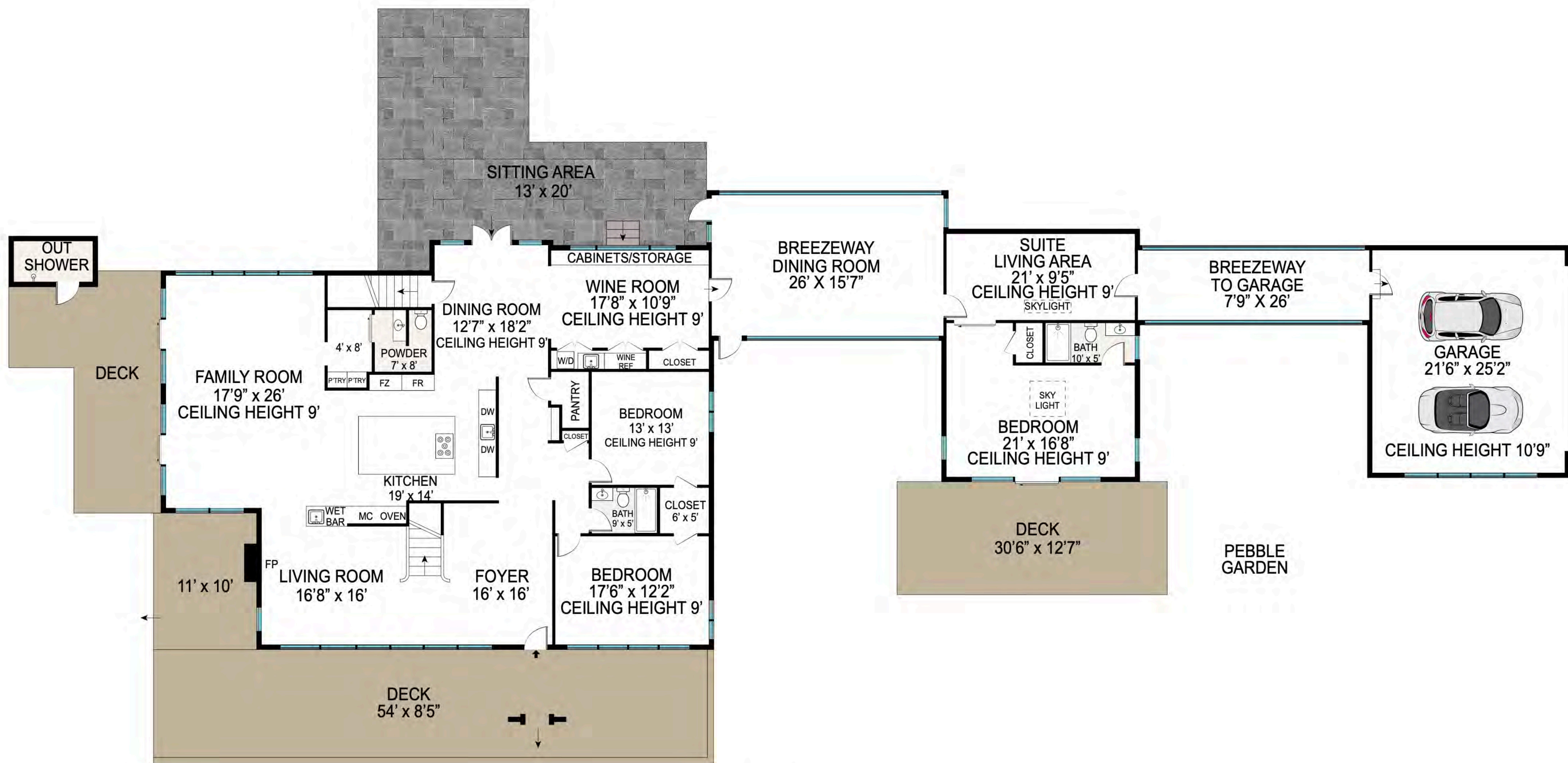
FIRST FLOOR CEILING HEIGHT: 9'
