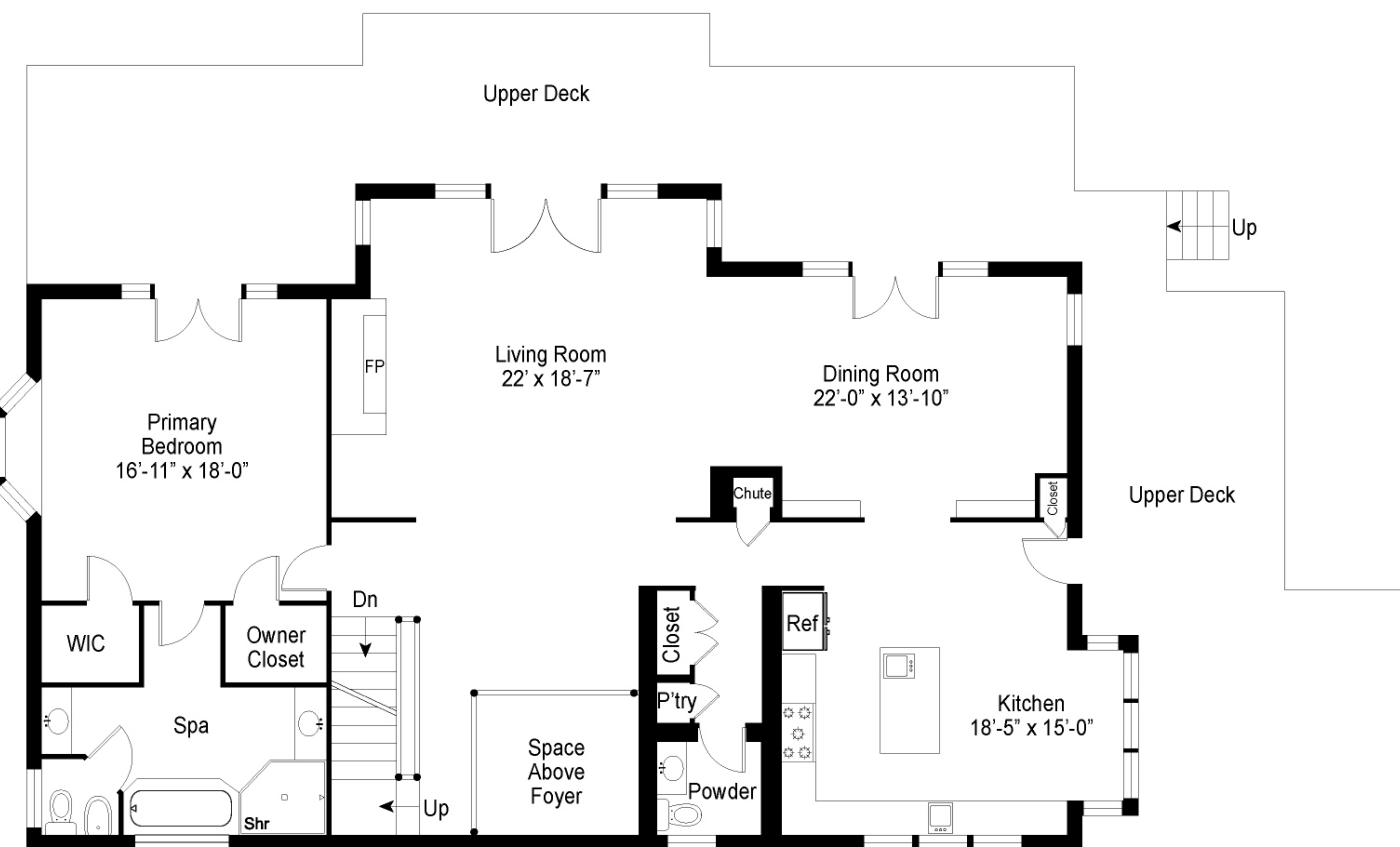
SECOND FLOOR
