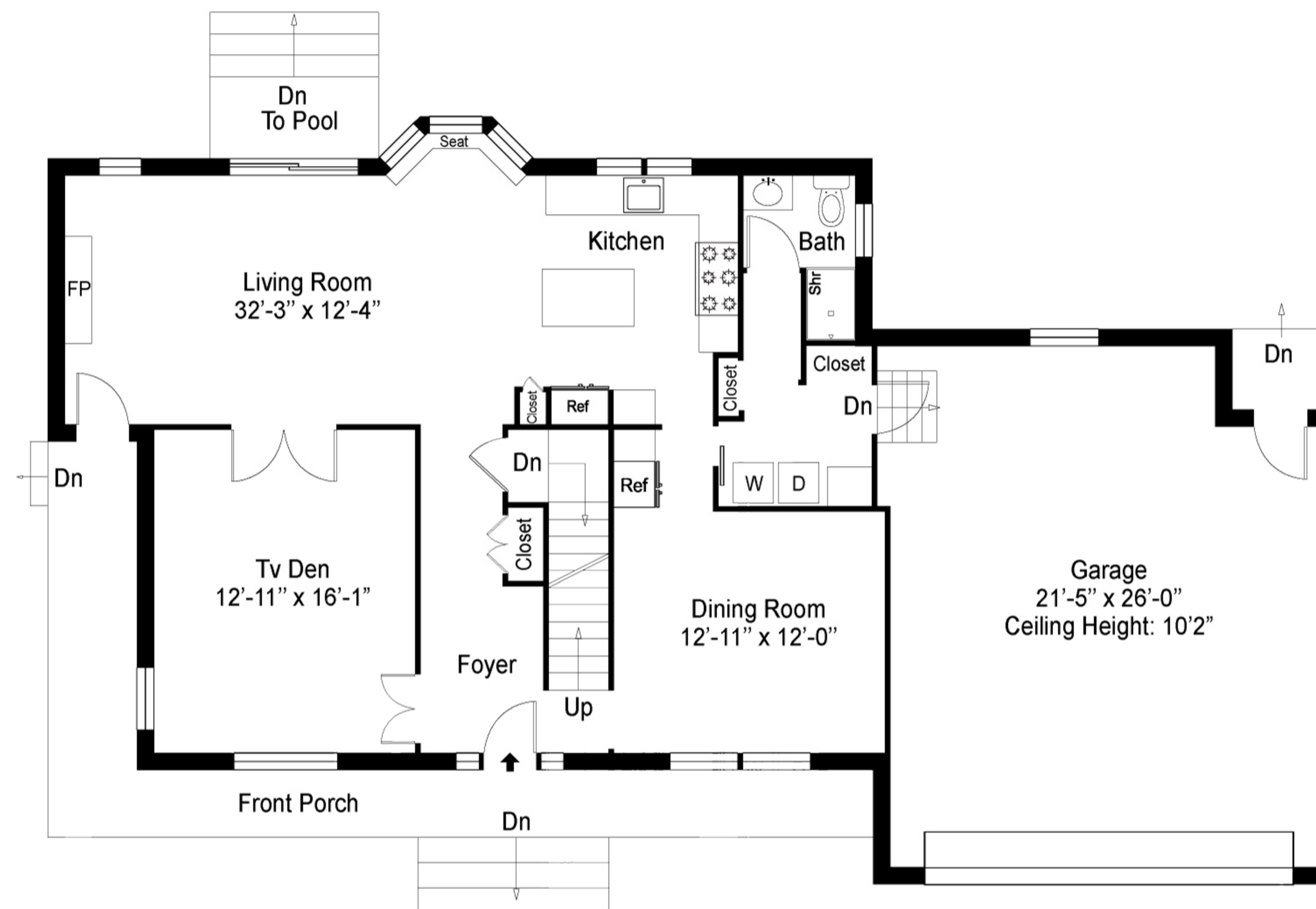
FIRST FLOOR
