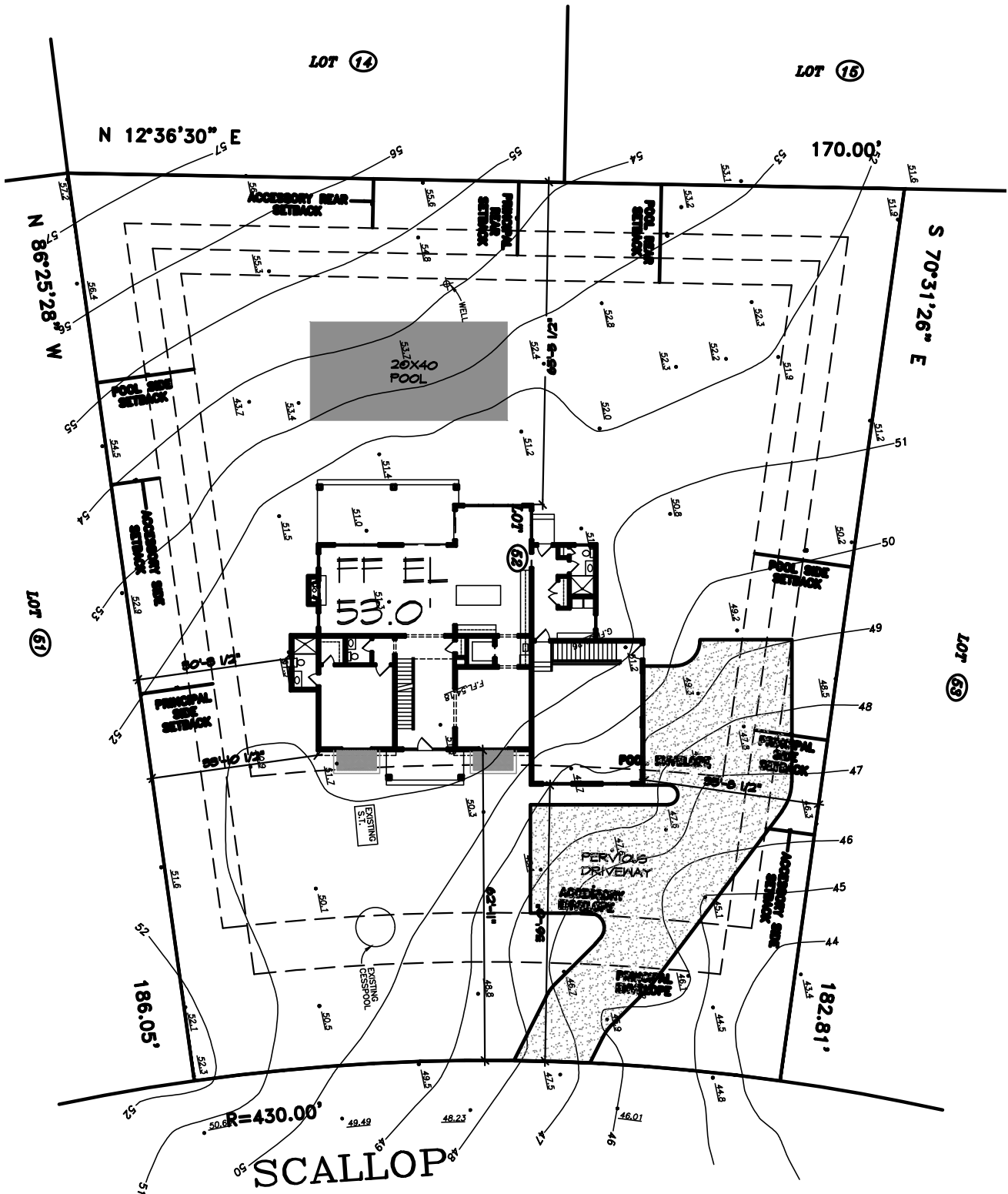
— PLOT PLAN
