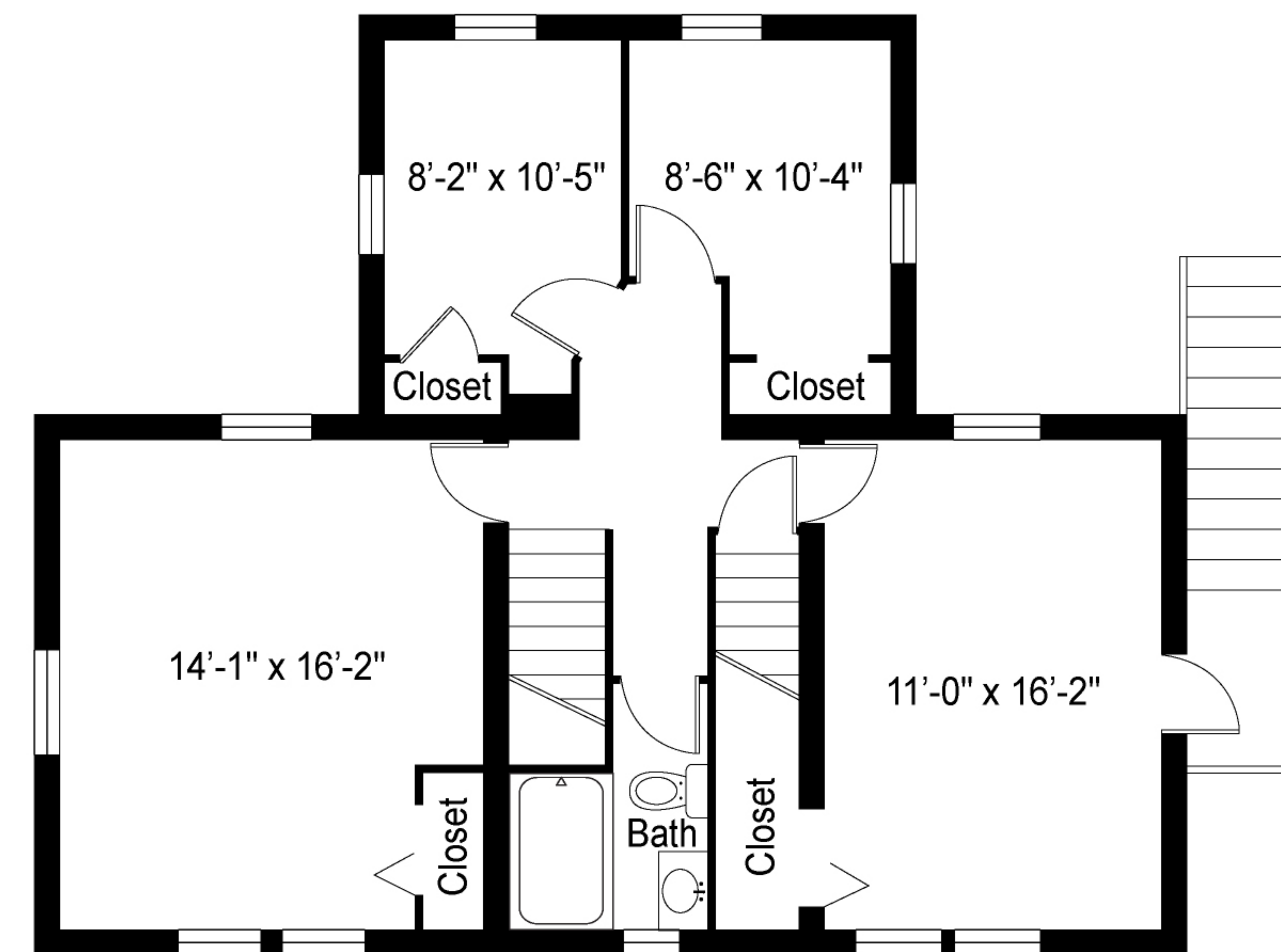
SECOND FLOOR
