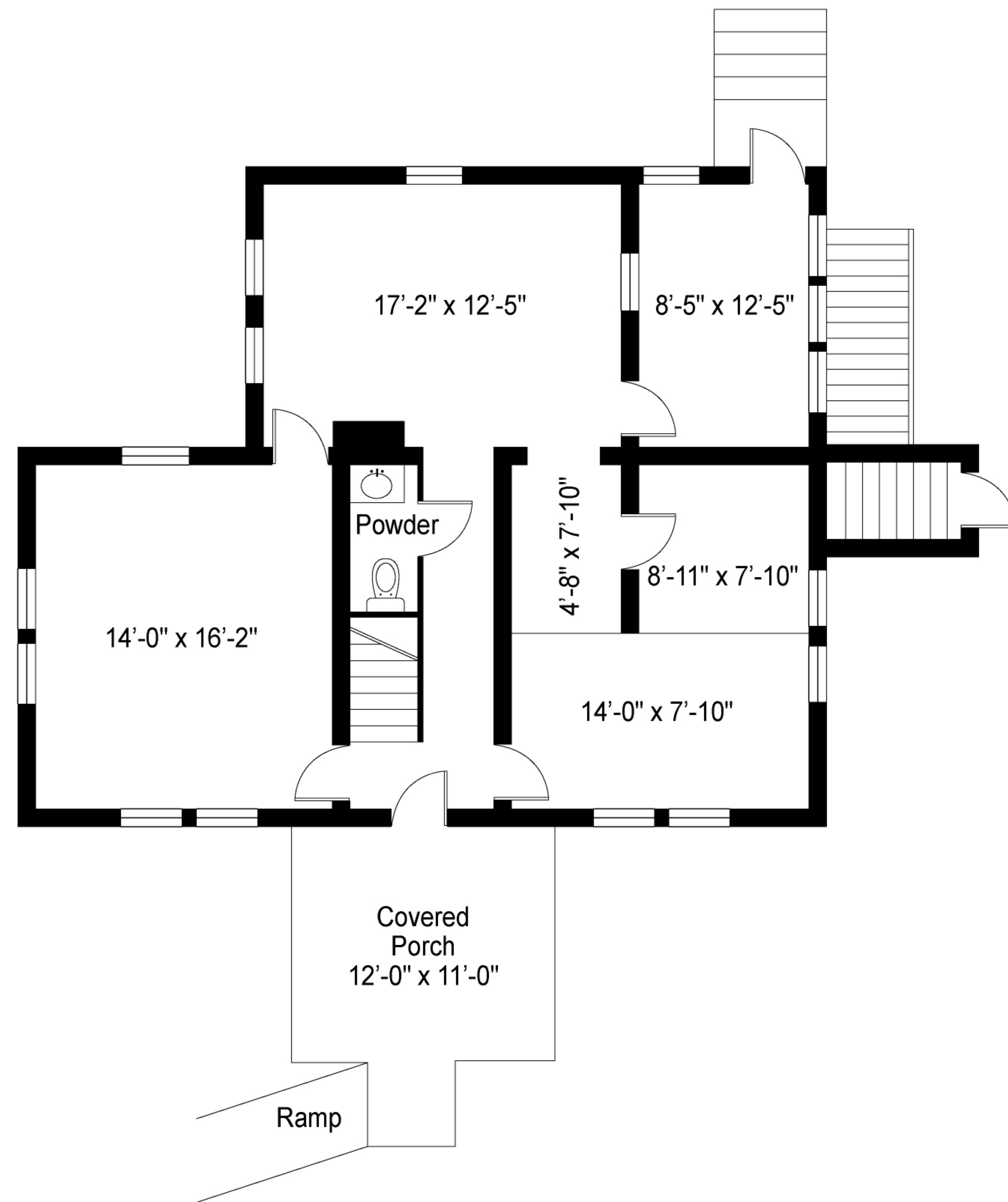
FIRST FLOOR
