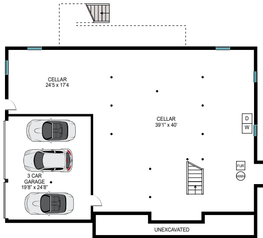
FOUNDATION PLAN
