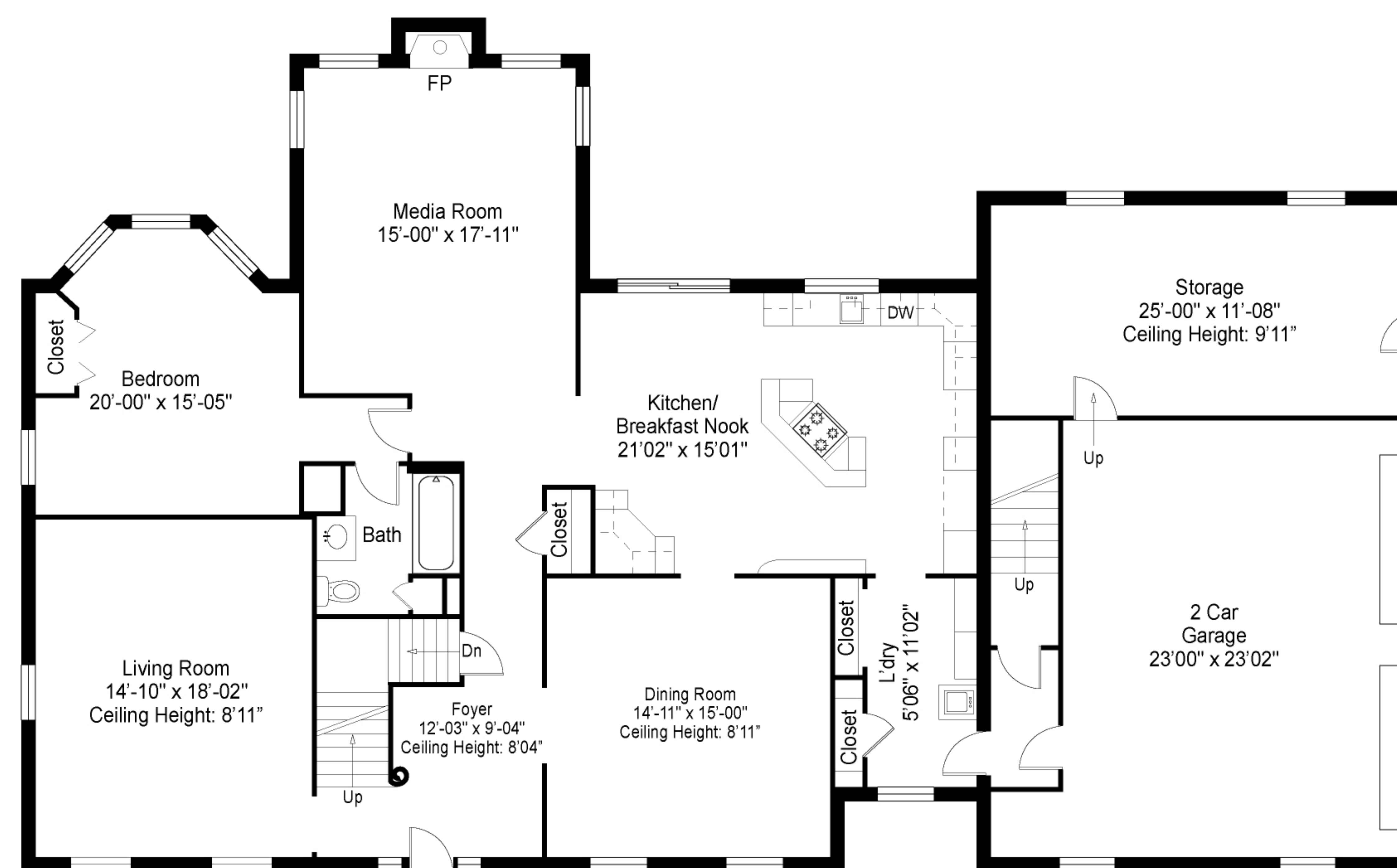
FIRST FLOOR
