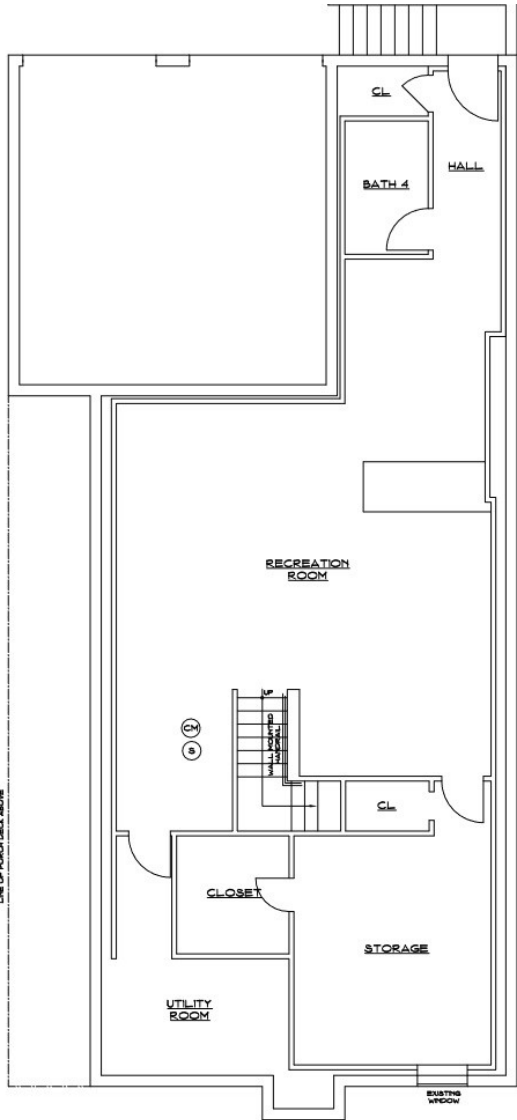
EXISTING BASEMENT FLOOR PLAN: 1/4" = 1' - 0"
