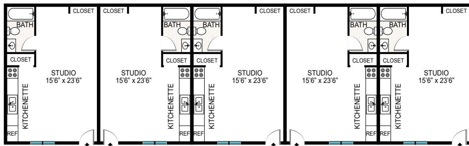
5 STUDIO UNITS INT: 1820 ft 2
