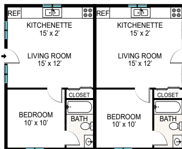
TYPICAL COTTAGE LAYOUT 2
