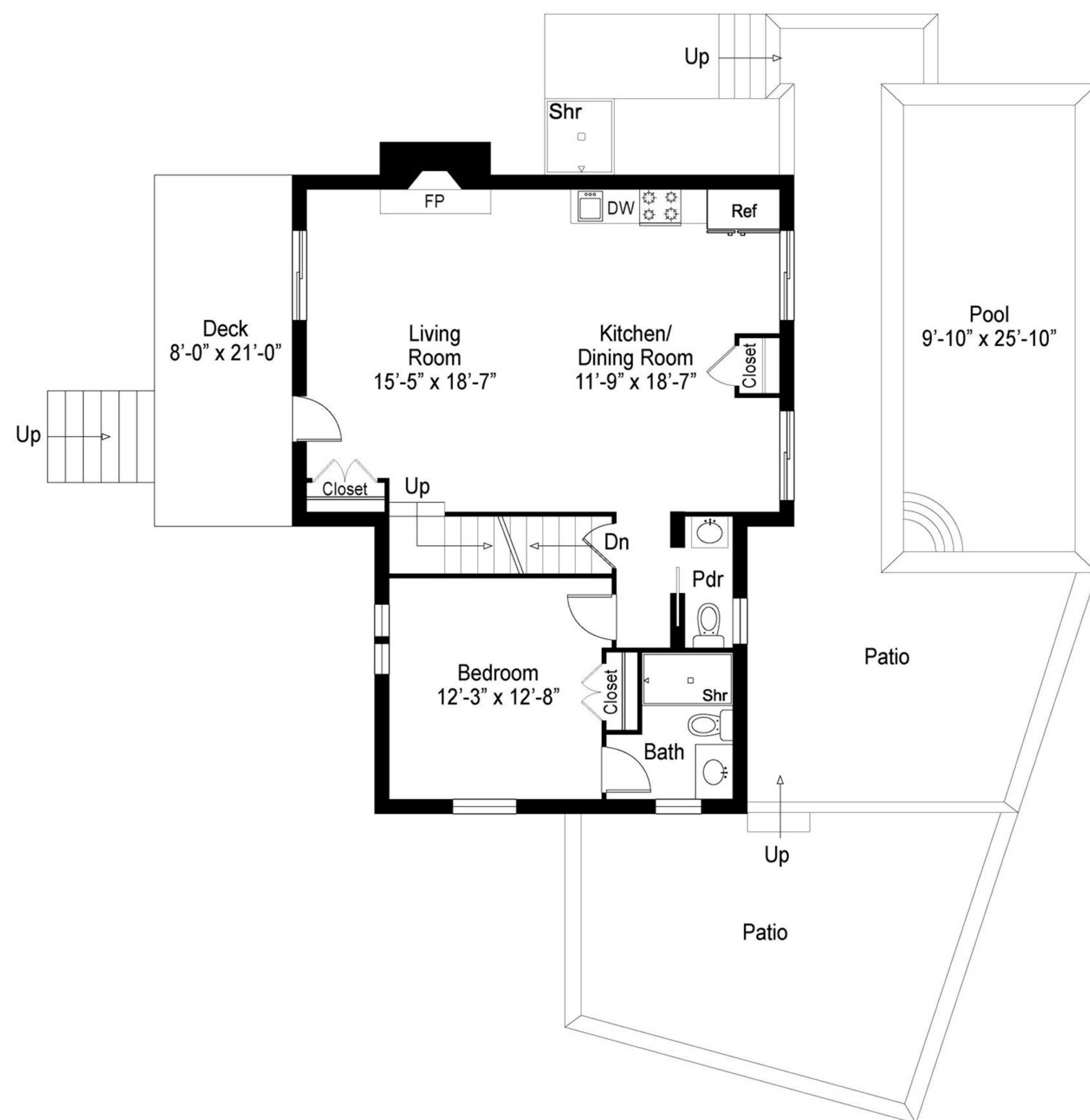
FIRST FLOOR
