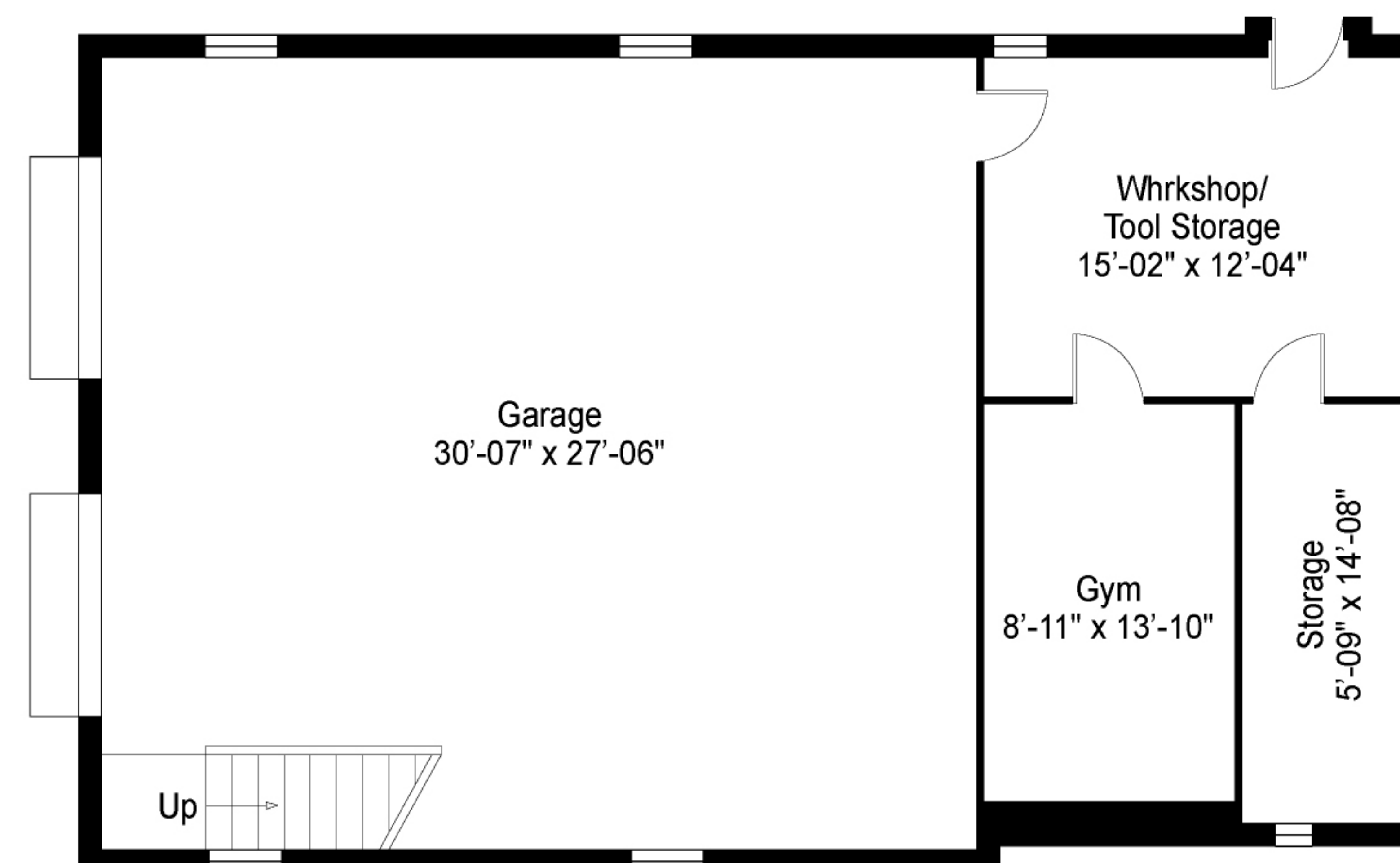
BASEMENT
