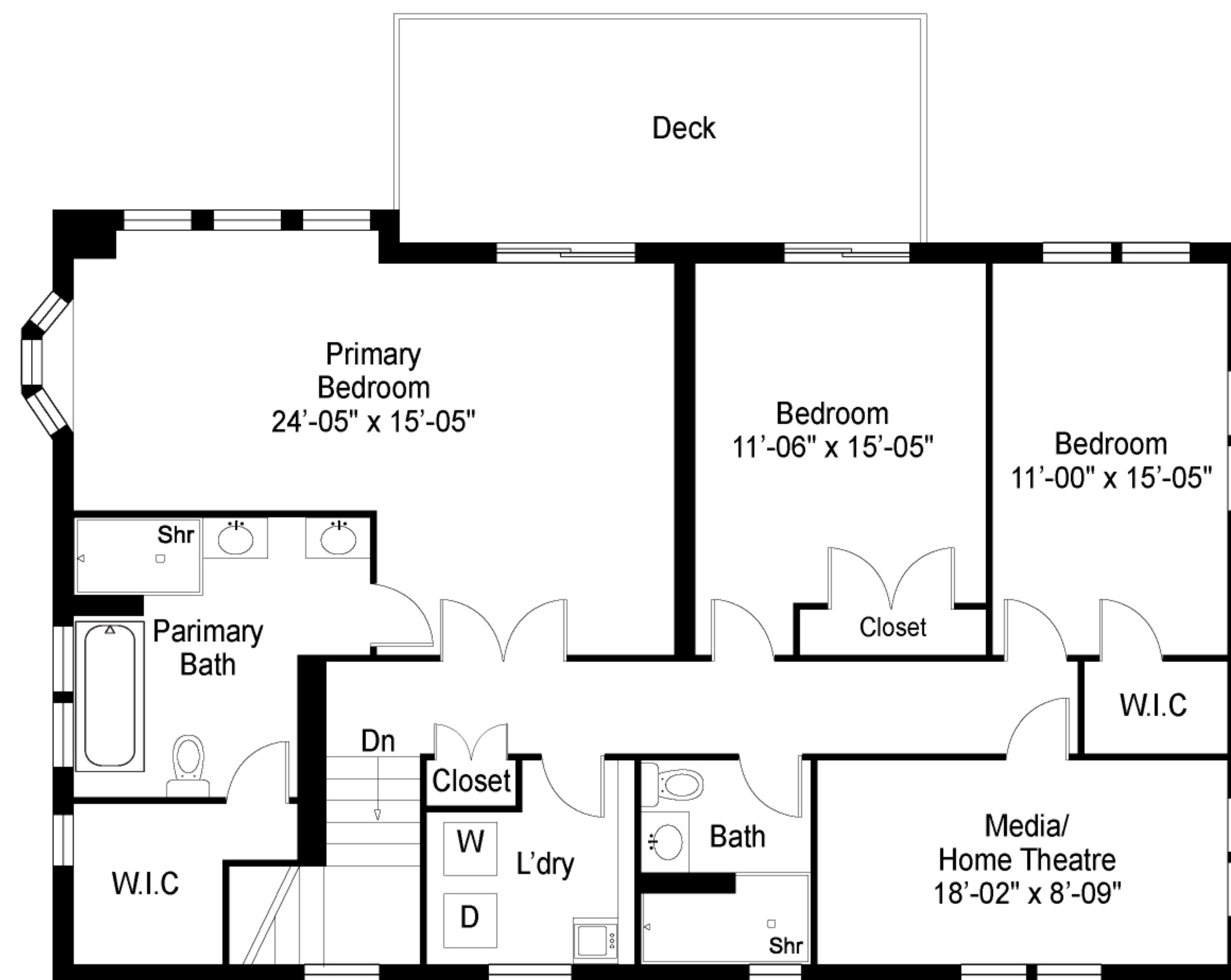
SECOND FLOOR
