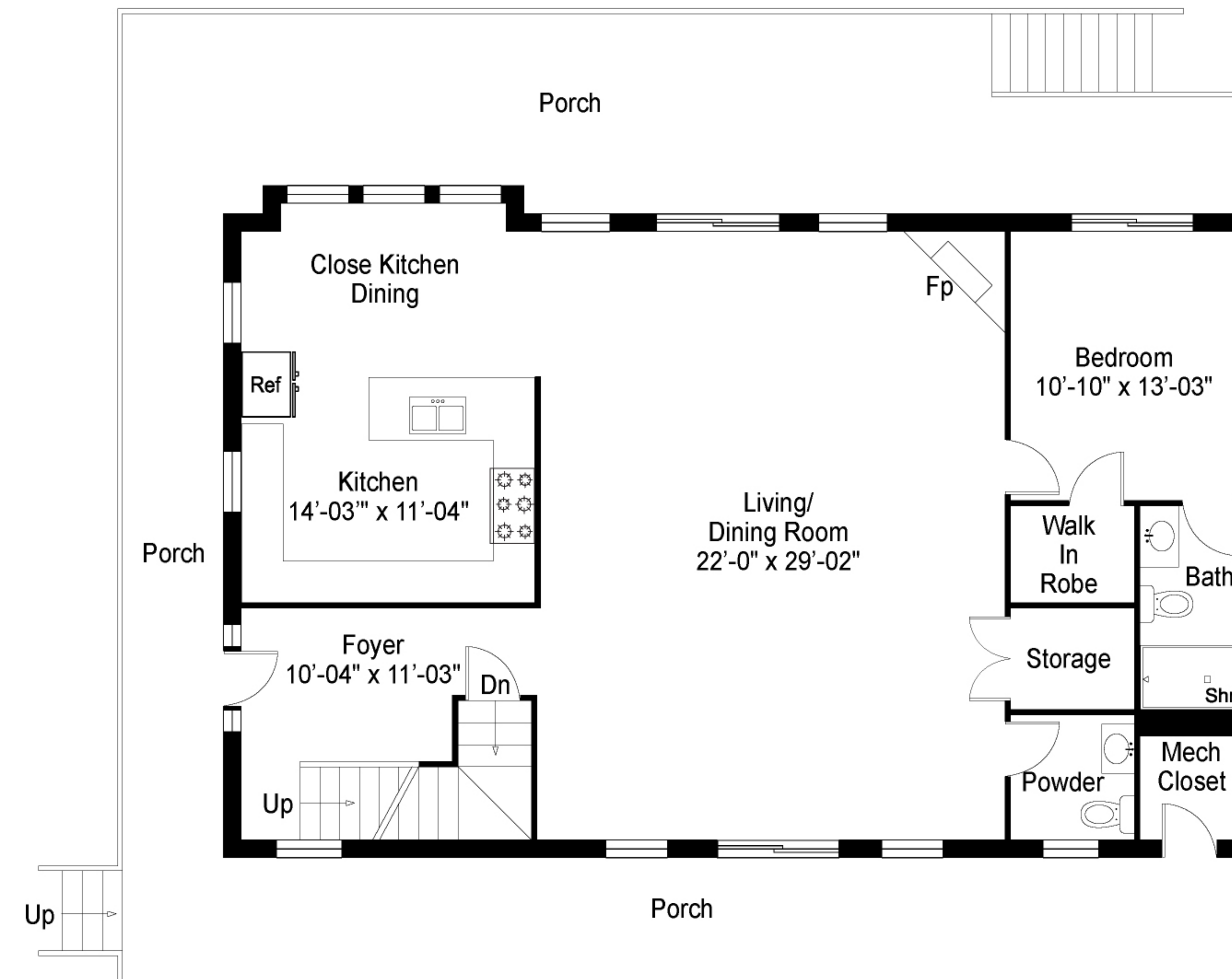
FIRST FLOOR
