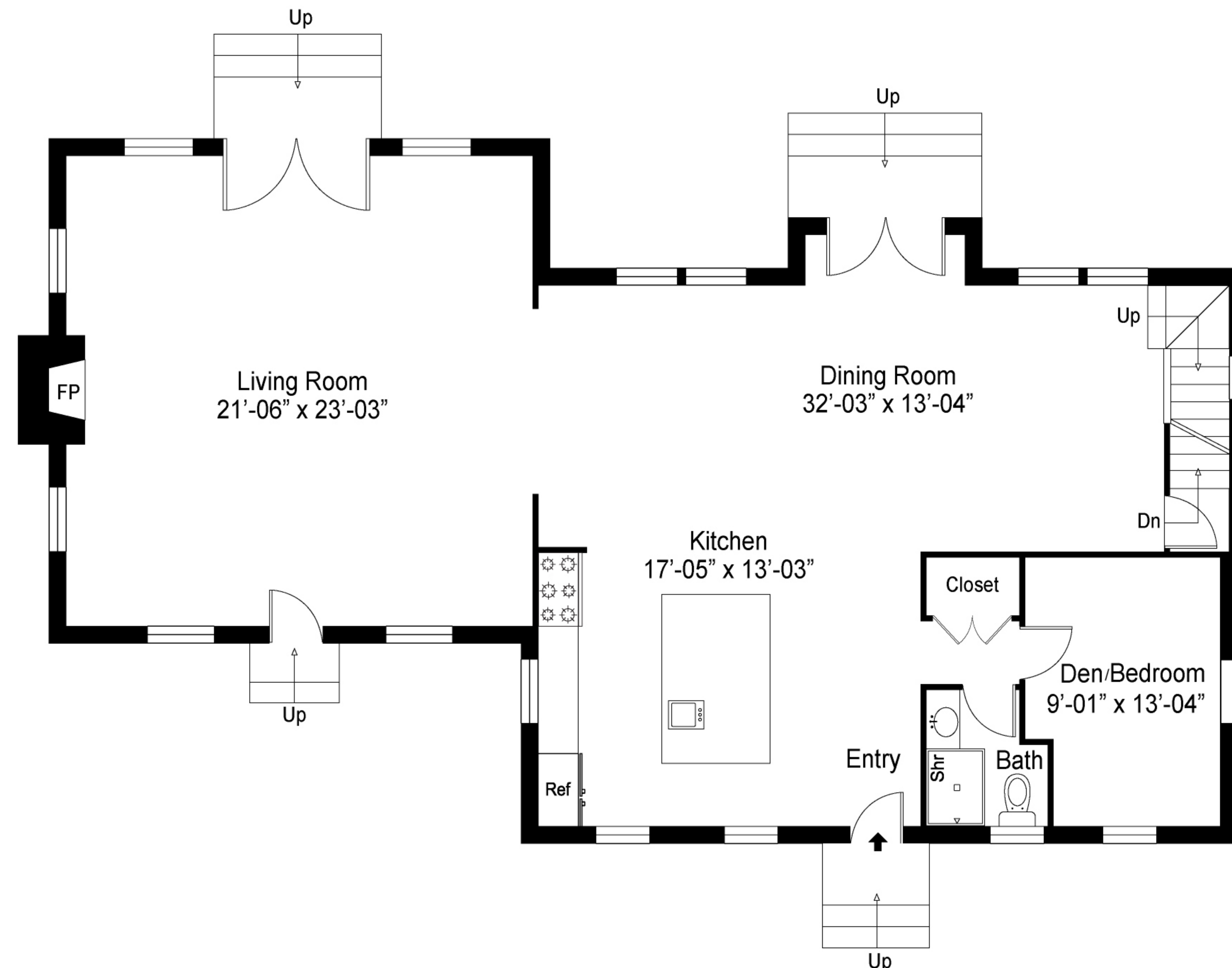
First Floor
