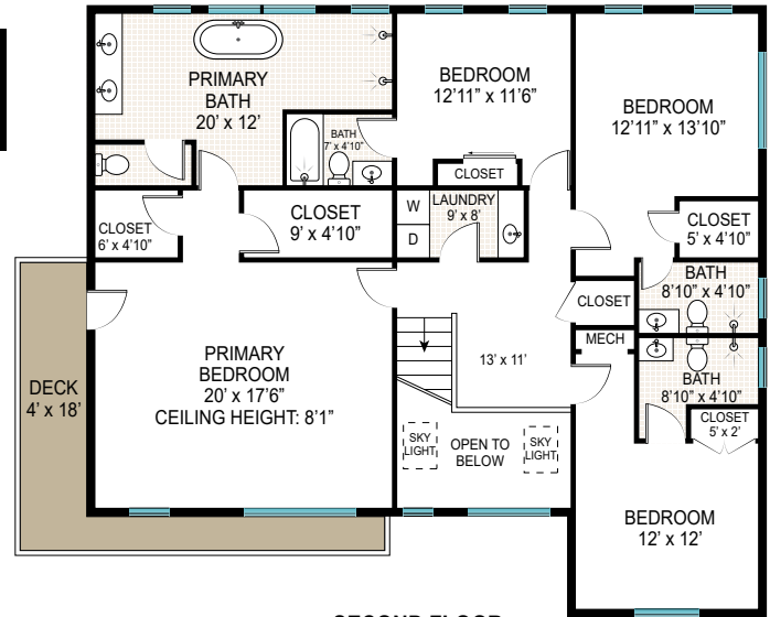
SECOND FLOOR
