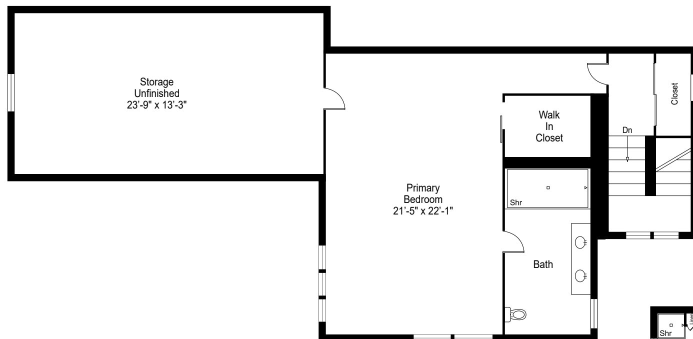
SECOND FLOOR
