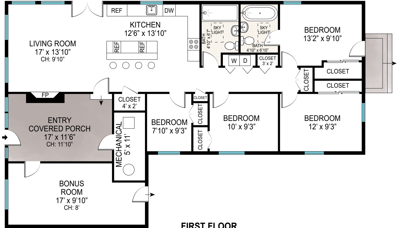
FIRST FLOOR CEILING HEIGHT: 9'10"
