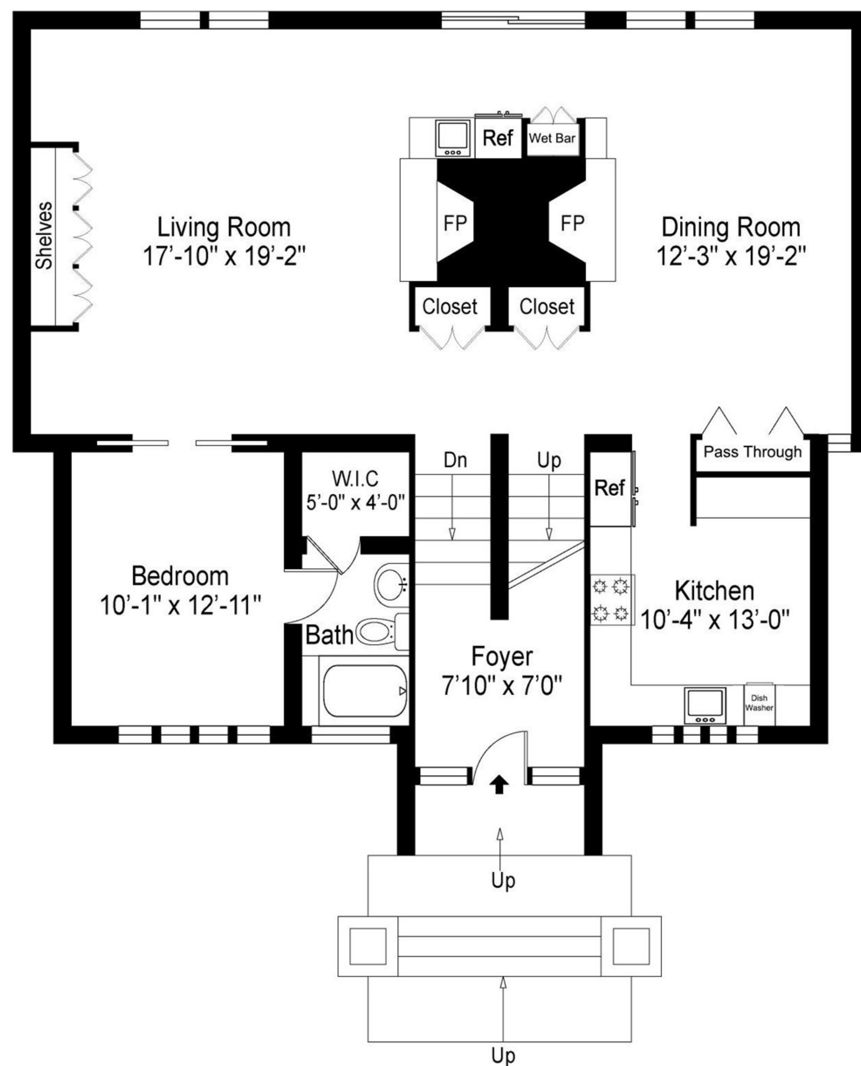
MAIN FLOOR
