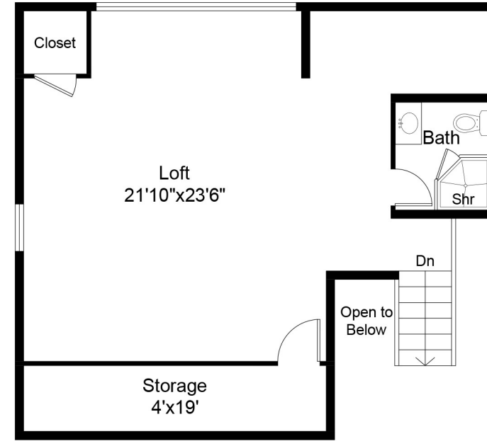
SECOND FLOOR PLAN NORTH WING
