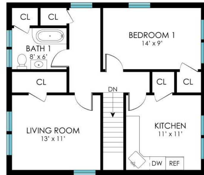
2ND FLOOR
