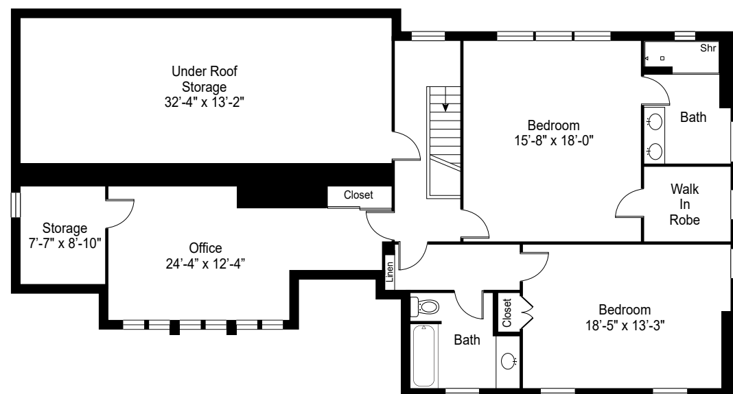
SECOND FLOOR
