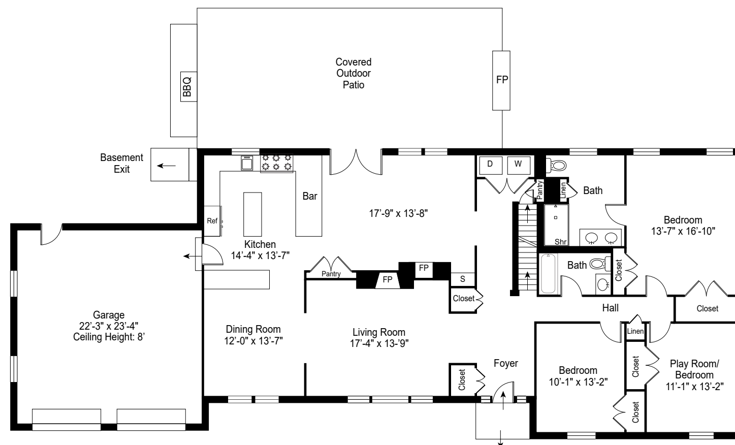
FIRST FLOOR
