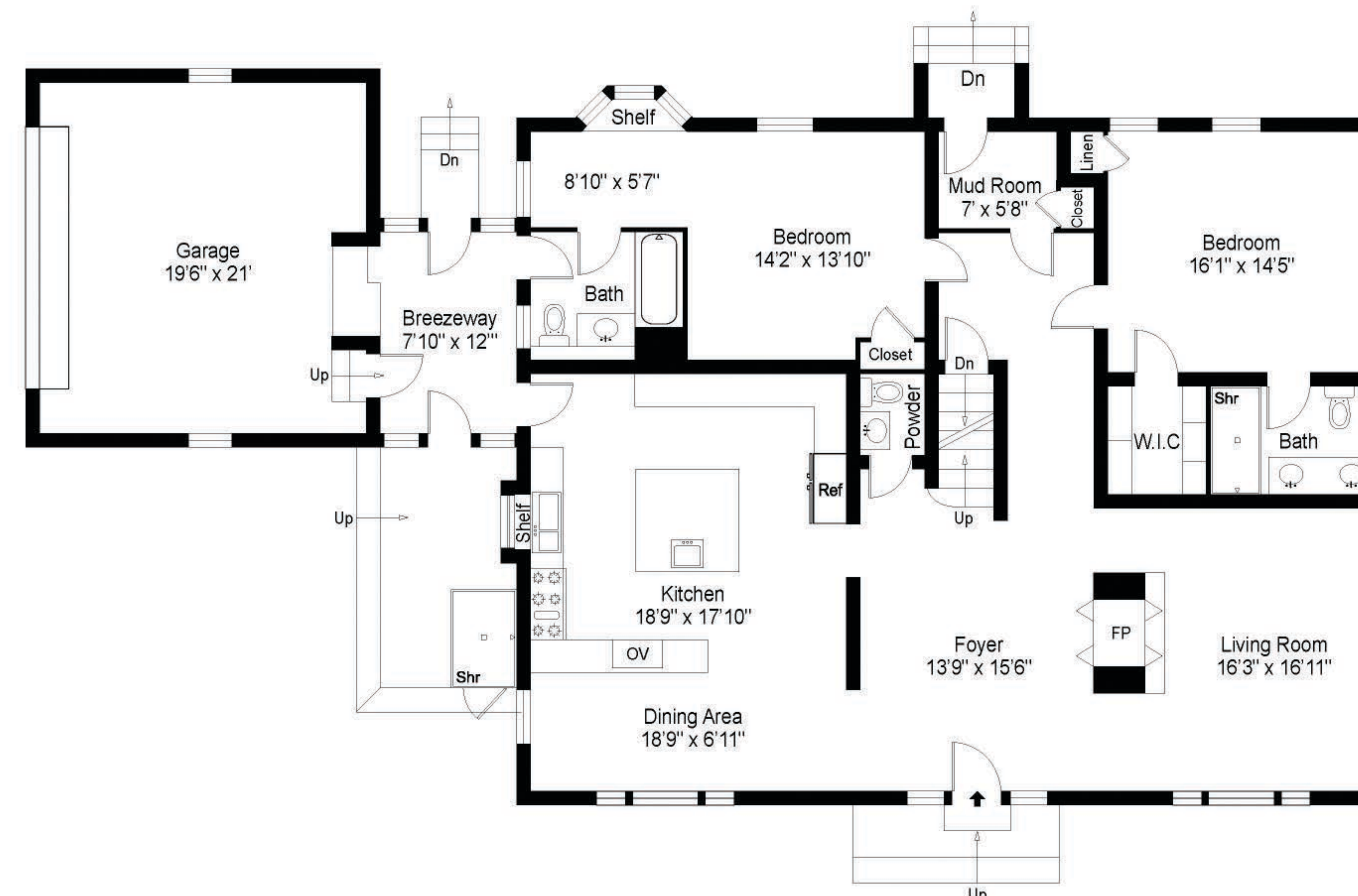
FIRST FLOOR
