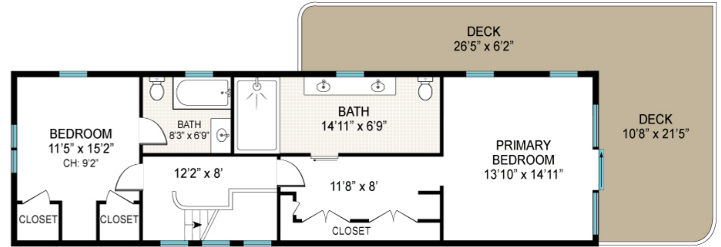
SECOND FLOOR CEILING HEIGHT: 9'2"
