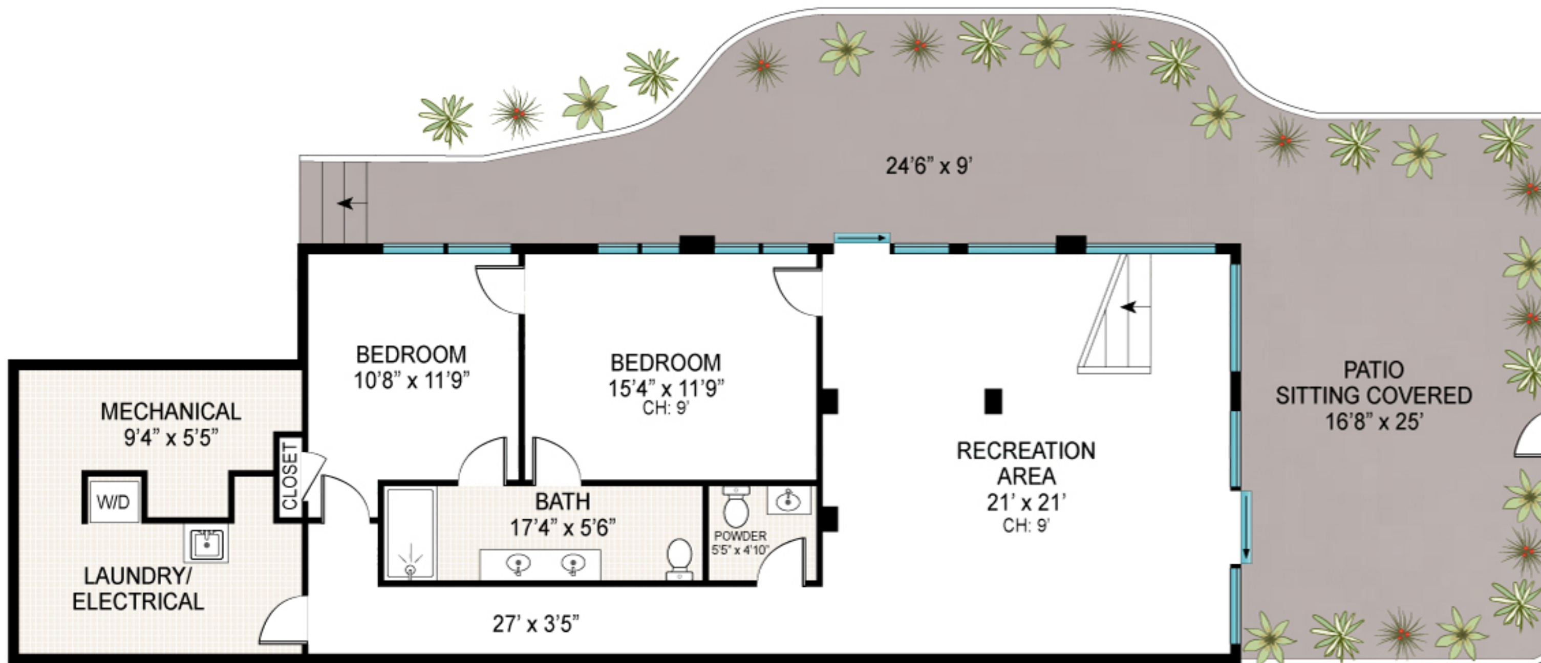
LOWER LEVEL CEILING HEIGHT: 9'
