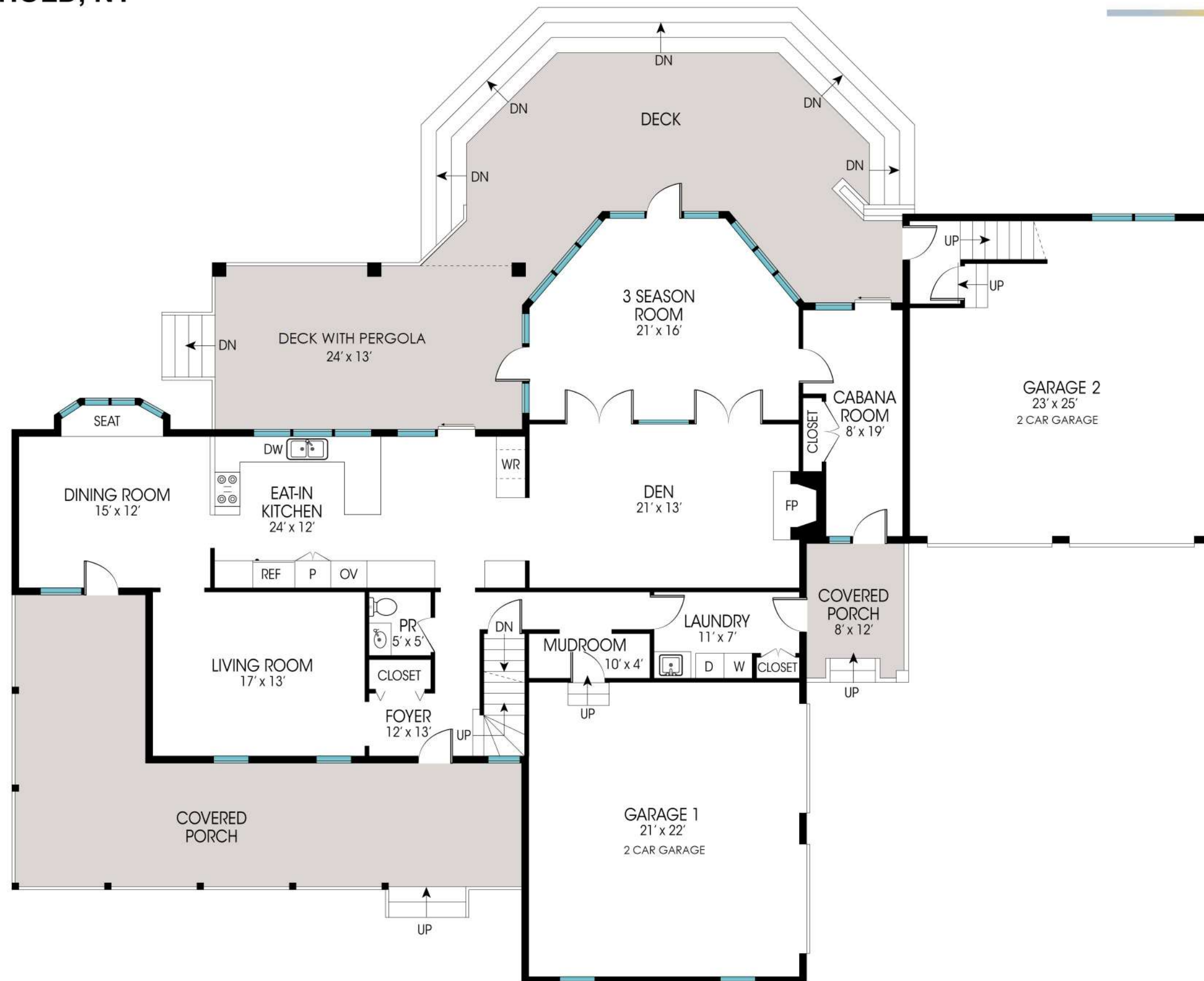
FIRST FLOOR
