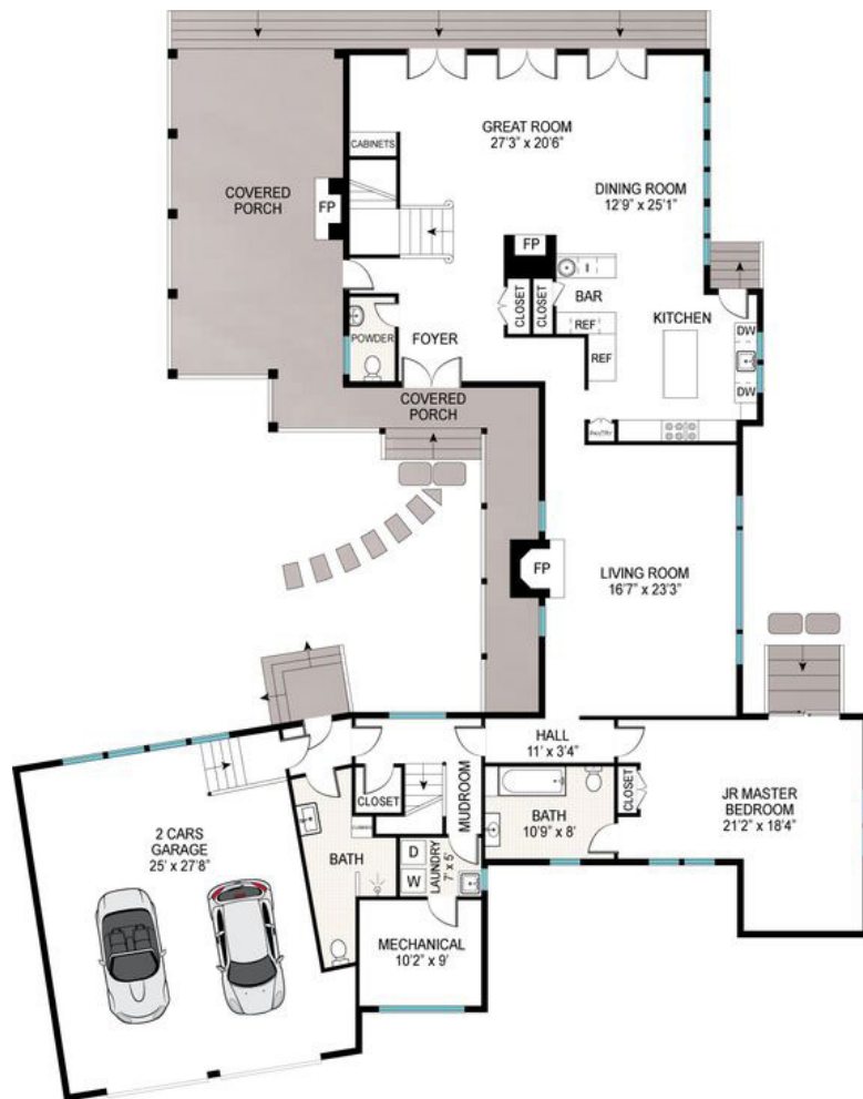
FIRST FLOOR INT. 2500 ft 2 EXT. 1225 ft 2 2 CARS GARAGE: 660 ft 2
