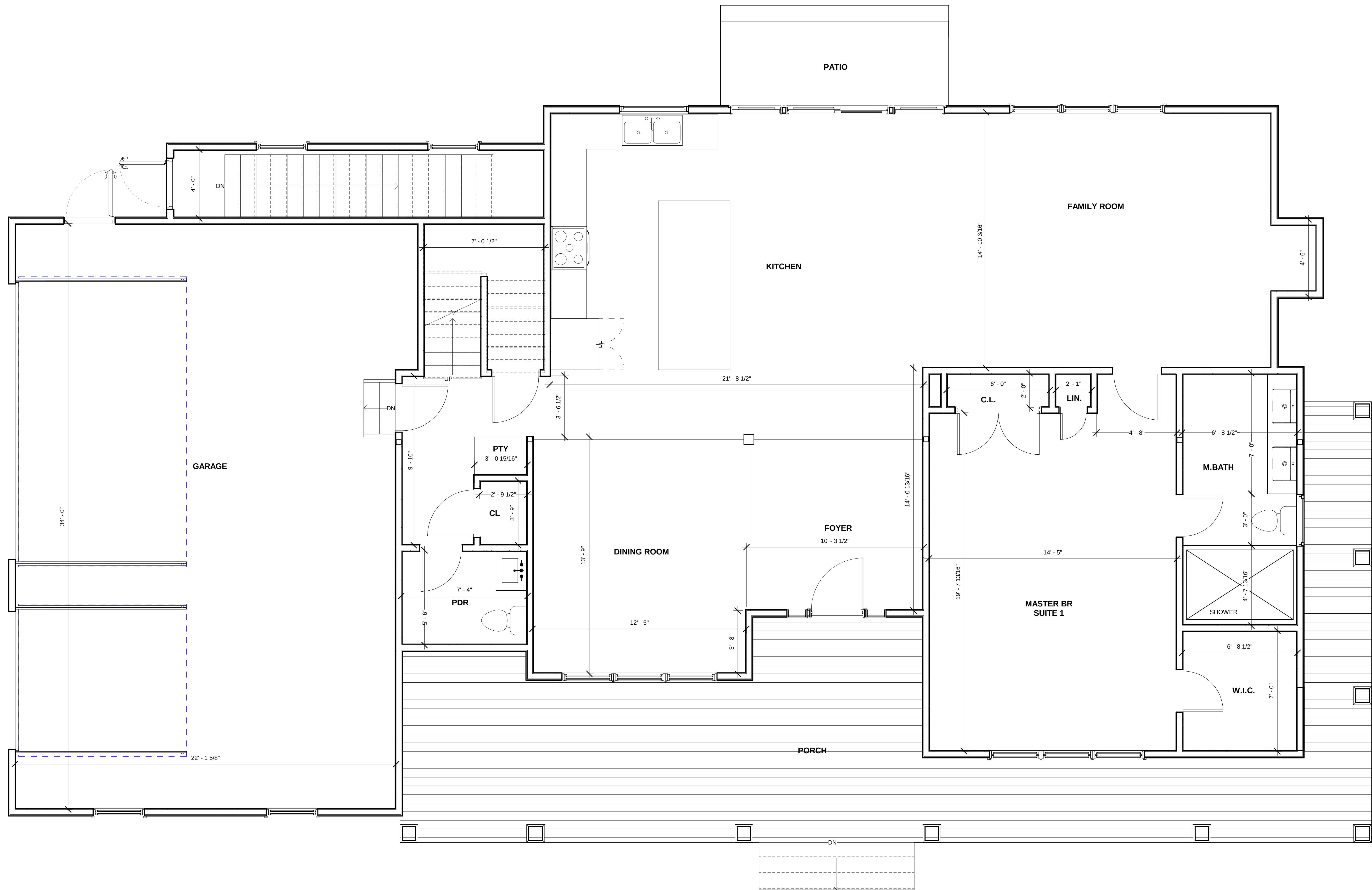
① 1ST FLOOR PLAN 3/8" = 1'-0"
