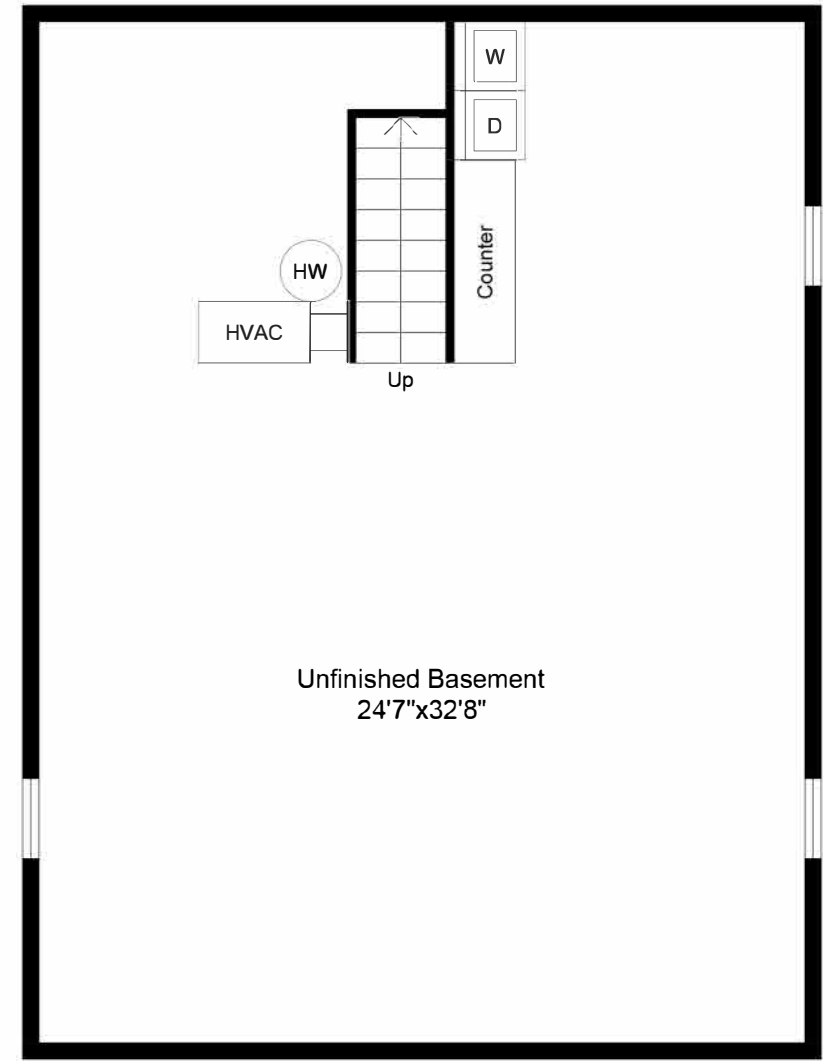
BASEMENT PLAN
