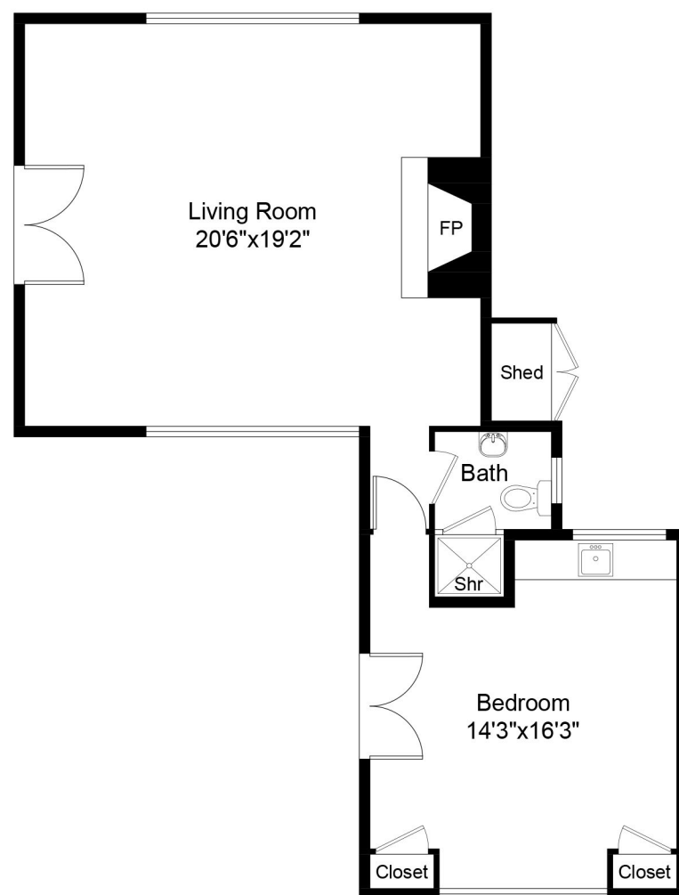
GUEST HOUSE FLOOR PLAN
