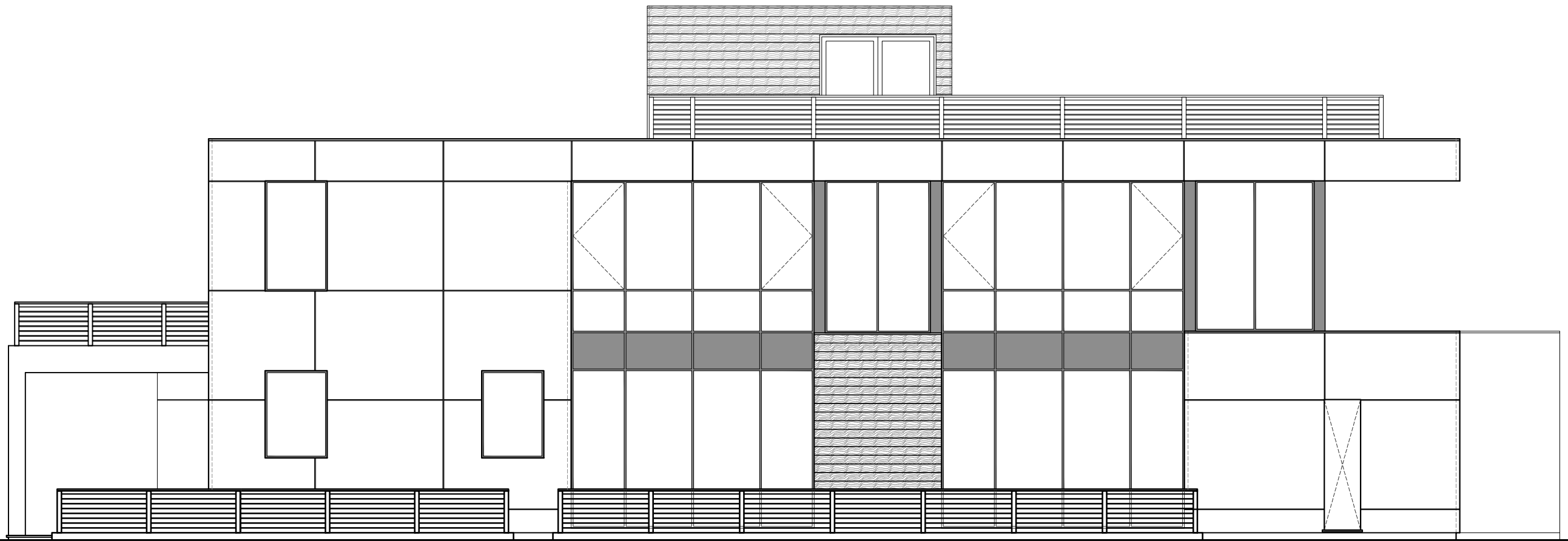
LEFT ELEVATION (11-20-20) 851 HALSEY LANE
