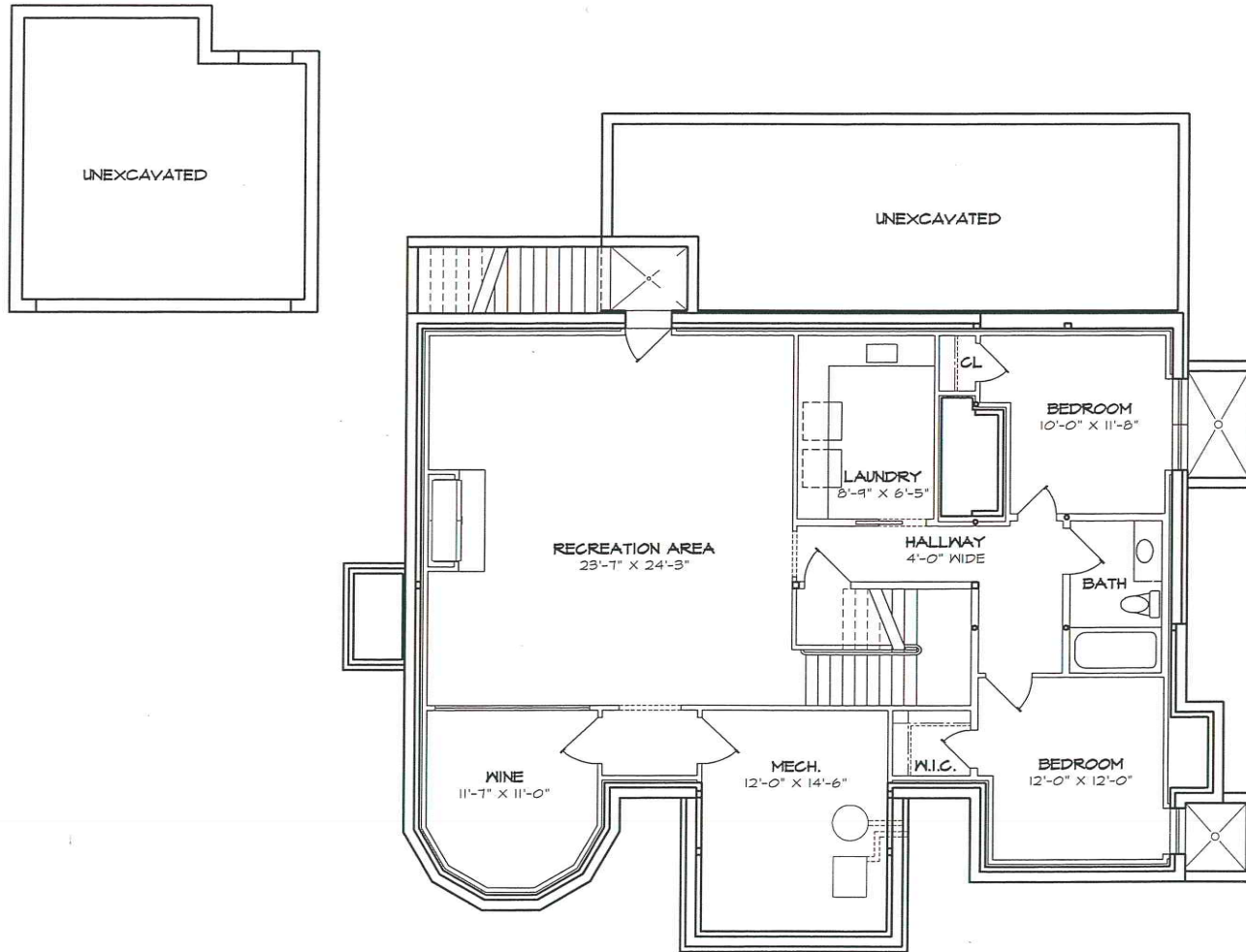
FINISHED BASEMENT PLAN
