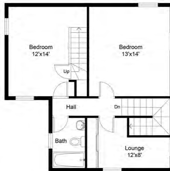
MAIN HOUSE SECOND FLOOR PLAN 500 sq.ft.
