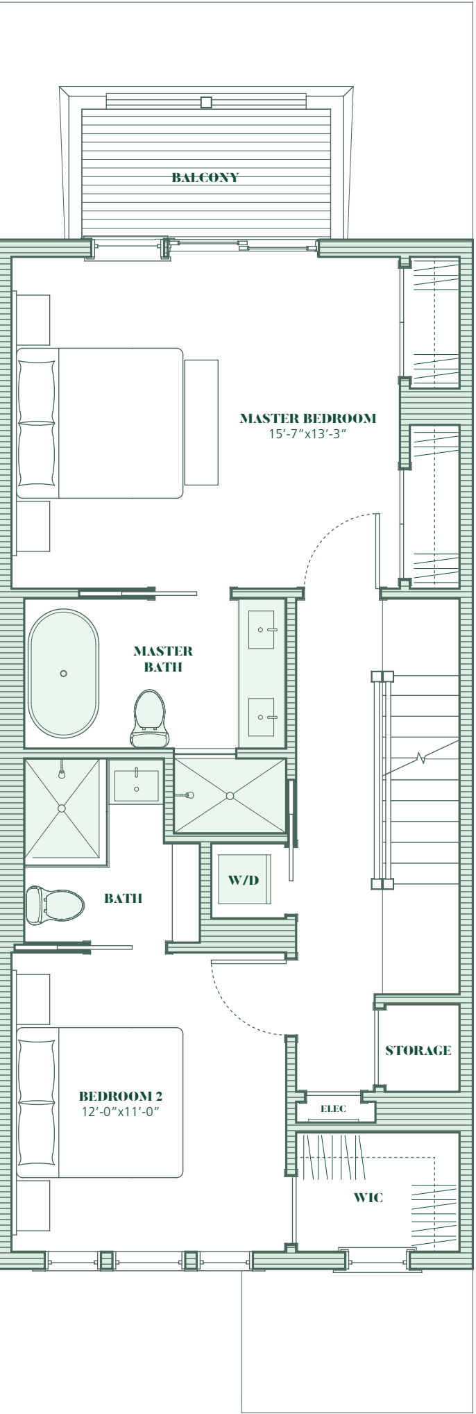
SECOND FLOOR
