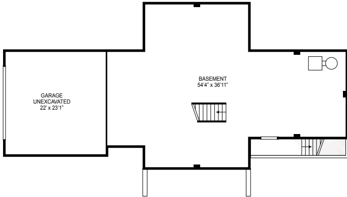
FOUNDATION PLAN
